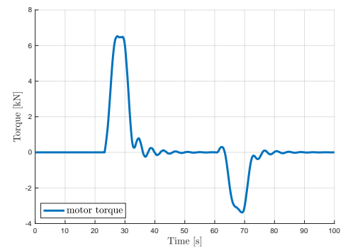
(f) MID algorithm: motor torque
