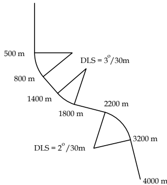
FIGURE 5: Wellbore survey of the well.
