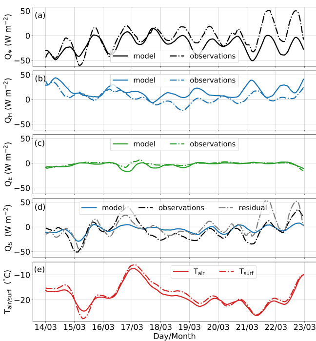
Figure 8. Comparison between observed and modeled hourly means of all constituents of the energy budget at the snow surface from 14 to 23 March 2020. The residual snow heat flux is obtained by subtracting the turbulent heat fluxes from the net radiation. Also shown are the air and surface temperatures during this period.
