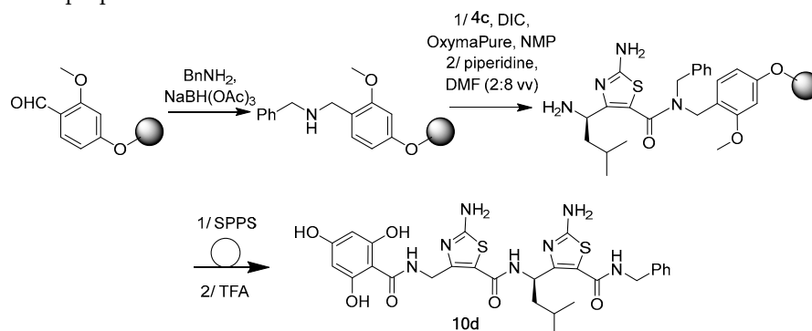
Scheme 3. Solid phase peptide synthesis (SPPS) approach to access ATC-based \gamma -peptide 10d .
