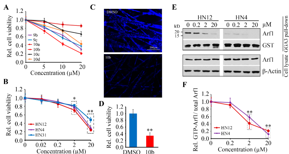
Figure 5. The anticancer effects of Arf1-targeting compounds. (A) The effects of Arf1-targeting compounds ( 9b , 9c , 10a , 10b , 10c , and 10d ) in a range dose from 0 to 20 \mu\text{M} on HN12 cell viability were determined by CellTiter-Glo ® Luminescent cell viability assay after 72 h treatment. (B) The dose-dependent cytotoxicity of compound 10b in three HNSCC cell lines (HN4, HN12, and HN31) was determined by CellTiter-Glo ® Luminescent cell viability assay after 72 h treatment. (C,D) The effects of 20 \mu\text{M} of compound 10b on HN12 cell viability in SeedEZ was determined after 72 h treatment. Representative images of DAPI staining and quantitative data of cell viability measured by alamarBlue are shown in (C) and (D) , respectively. (E,F) Arf1 protein levels and its activity in HN12 and HN4 cells treated with or without compound 10b were determined by GGA3 pull-down assay and Western blotting. A representative result and quantitative data from three independent experiments are shown in (E) and (F) , respectively. * p < 0.05 ; ** p < 0.01 .
