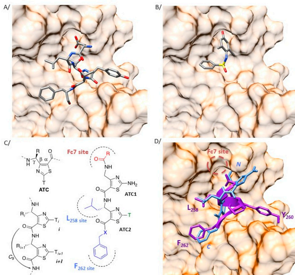
Figure 2. Heteroaromatic \gamma -dipeptide to mimic the auto inhibitory domain of cytohesin proteins.
