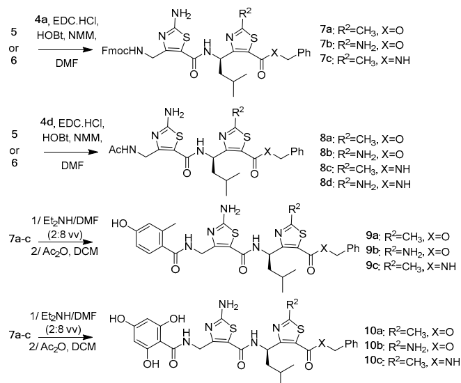
Scheme 2. Synthesis of the ATC-based \gamma -dipeptides.
