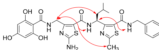
Figure 4. Characteristic nuclear overhauser effect (NOE) correlations observed for typical constrained \gamma -peptidic dimer 10c .
