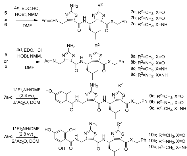
Scheme 2. Synthesis of the ATC-based \gamma -dipeptides.
