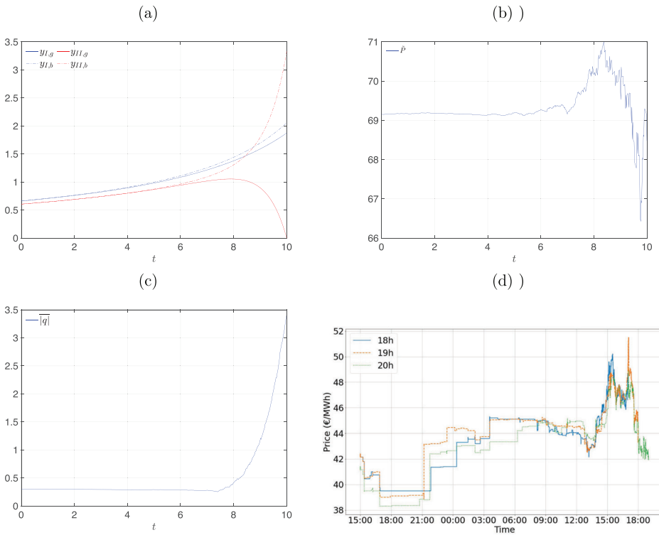
FIGURE 2 (a) The functions y_{I,g} , y_{I,b} , y_{II,g} , and y_{II,b} , in (b) the approximated market equilibrium price and in (c) a measure of the trading activity given by \frac{1}{N} \sum_i |q_t^i| . Parameters value: N_I = 100 , \lambda_I^g = 0.1 , \lambda_I^b = 0.1 , \beta_I^g = 6 , \beta_I^b = 7 , \mu_I = 0 ; N_{II} = 100 , \lambda_{II}^g = 0.5 , \lambda_{II}^b = 0.5 , \beta_{II}^g = 0 , \beta_{II}^b = 20 , \mu_{II} = 0 ; \gamma_I = \gamma = 10 , \eta_I = \eta = 10 , d_0^i = 20 . (d) Intraday mid-prices on EEX market on August, 30th, 2017 for deliveries at 18, 19, and 20 h up to 1 h before maturity, picture extracted from Deschatre and Gruet (2021) with the permission of the authors [Color figure can be viewed at wileyonlinelibrary.com]
