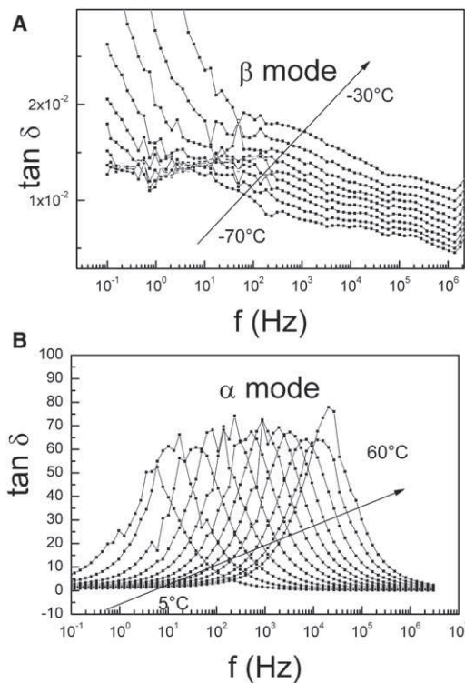
FIGURE 8 DDS isotherms of purified supernatant from control VSMCs. (A) The \beta -mode between -70^{\circ}\text{C} and -30^{\circ}\text{C} . (B) The \alpha -mode between 5^{\circ}\text{C} and 60^{\circ}\text{C} .
