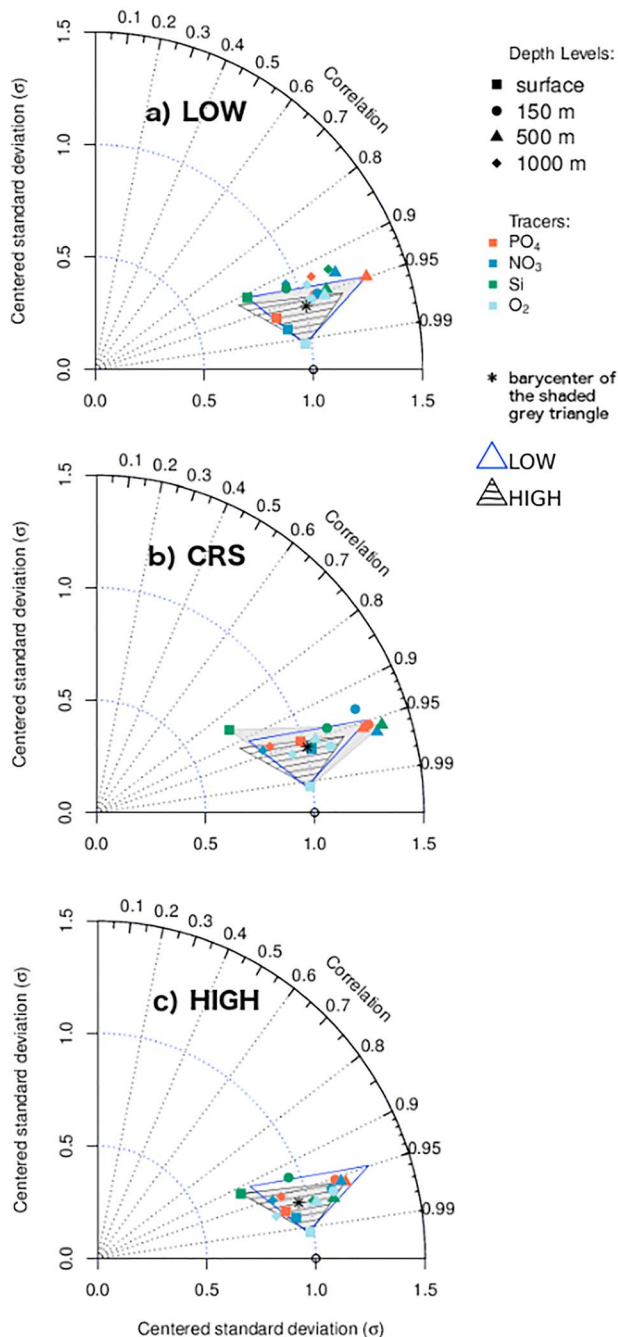
Figure 12. Taylor diagrams showing the correspondence of global annual mean distributions of \text{PO}_4 (red), \text{NO}_3 (blue), Si (green), and \text{O}_2 (cyan) between observations and (a) LOW, (b) CRS, and (c) HIGH. Shapes and colors of the symbols are indicative of the considered depth level and tracer, respectively. The shaded grey triangle represents the mean skill score characteristics of the considered experiment. Its coordinates on the angular axis are the maximal correlations, the correlation at the maximal standard deviation, and the correlation at the minimal standard deviation. On the radial axis, its coordinates are the standard deviation at the maximal correlation, the maximal standard deviation, and the minimal standard deviation. The blue (black hatched) polygon superimposed on each Taylor diagram is indicative of the skill of LOW (HIGH, respectively).
