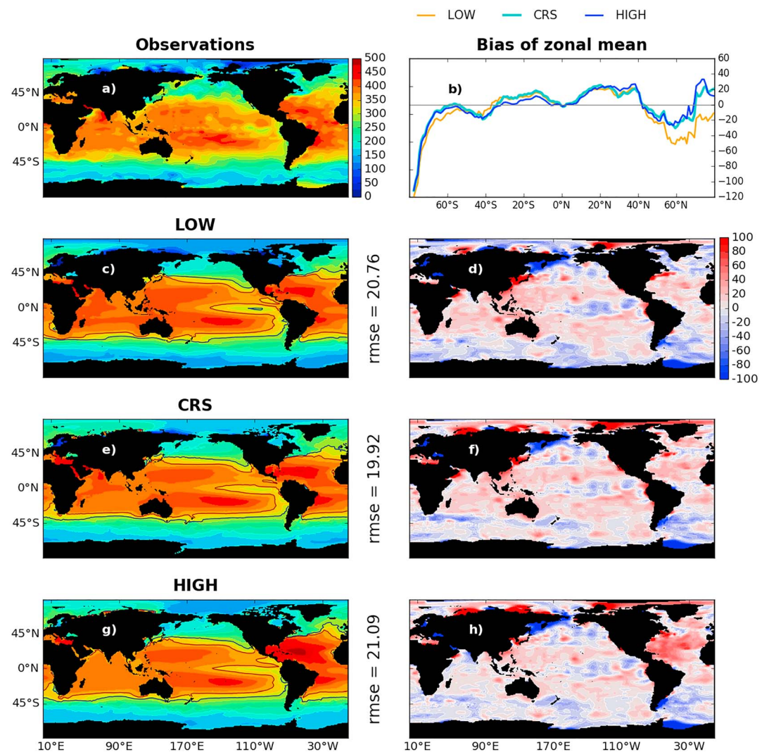
Figure 11. Idem Figure 8 for Alk-DIC concentration ( \text{mmol/m}^3 ), except that no stippling has been added on subfigure (f). Black contours highlight fronts of concentration equal to 300 and 350 \text{mmol/m}^3 .
