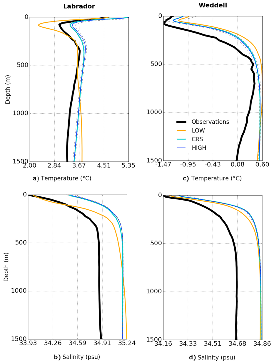
Figure 4. Mean modeled and observed annual vertical profiles of temperature (°) and salinity (psu) within (a, b) the Labrador Sea [55°W–45°W, 50°N–60°N] and (c, d) the Weddell Sea [55°W–45°W, 70°S–60°S] over the 2000–2009 period. Gray dashed lines correspond to the confidence interval at 95% of HIGH mean profiles.
