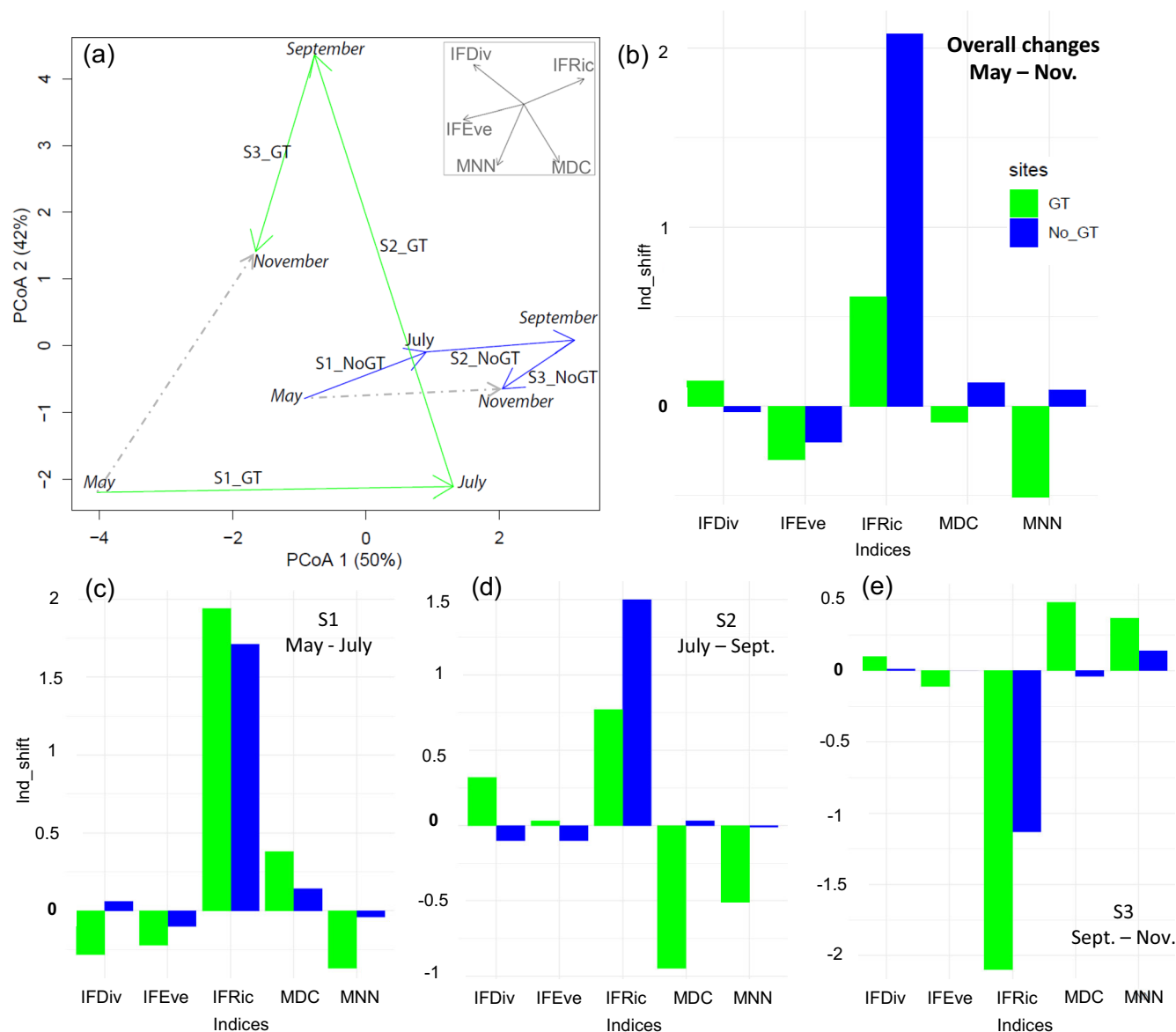
FIGURE 7 Structural and functional trajectories at impacted (green) and pristine (blue) beaches. (a) Trajectory diagram in \Omega_7 space. Only two dimensions are shown, representing 92% of the total variance. Solid lines ending with an arrow represent segment lengths and dotted arrow net changes. (b–e) Bar plots represent the shift in value of five structural and functional indices: isotopic functional richness (IFRic), evenness (IFEve), divergence (IFDiv), and mean distance to nearest neighbor (MNN), and centroid (MDC). Bar plot panels show changes in indices values between May and November (b) and for all pairs of consecutive periods (c: May to July, d: July to September, e: September to November). Data from Quillien et al. (2016)
