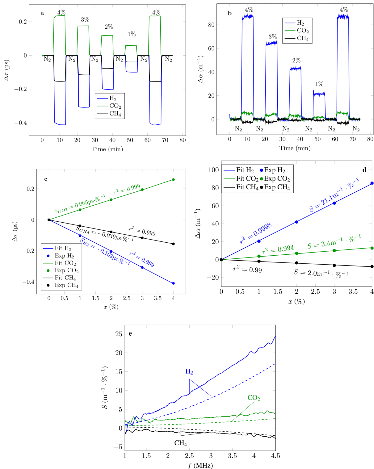
Figure 2. Sensor response to binary mixtures of \text{N}_2 with either \text{H}_2 , \text{CO}_2 or \text{CH}_4 . (a) Shift in time of flight when alternating the mixture at different concentrations with pure \text{N}_2 . (b) Attenuation shift at 4 MHz when alternating the mixture at different concentrations with pure \text{N}_2 . (c) Calibration curves from (a) . (d) Calibration curves from (b) . (e) Experimental (solid lines) and theoretical (dashed lines) values of the sensor sensitivity in attenuation shift as a function of the excitation frequency for the three binary gas mixtures.
