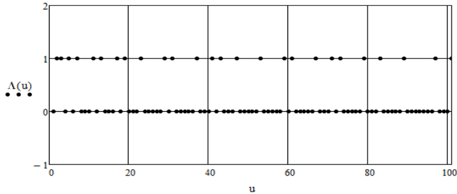
Fig 1 Plot of the prime discriminating function \Lambda in the integer interval [1, 101] . The 26 primes in that domain appear plotted (dots) along the straight line \Lambda(u)=1 , the remaining integers in that domain appear on the abscissa axis.
