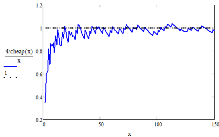
Fig. 13 The function \Psi_{Cheapp}(x)/x plotted in the integer interval (2, 150) showing its asymptotic behaviour towards its limit 1 (equivalent to verifying the prime number theorem)
