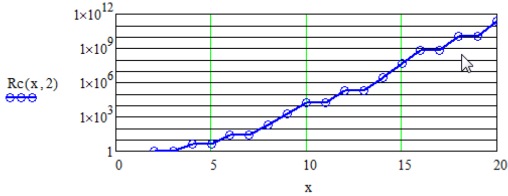
Fig. 12 Plot of the product R_c of the composite numbers in the integer domain (2, 20)
