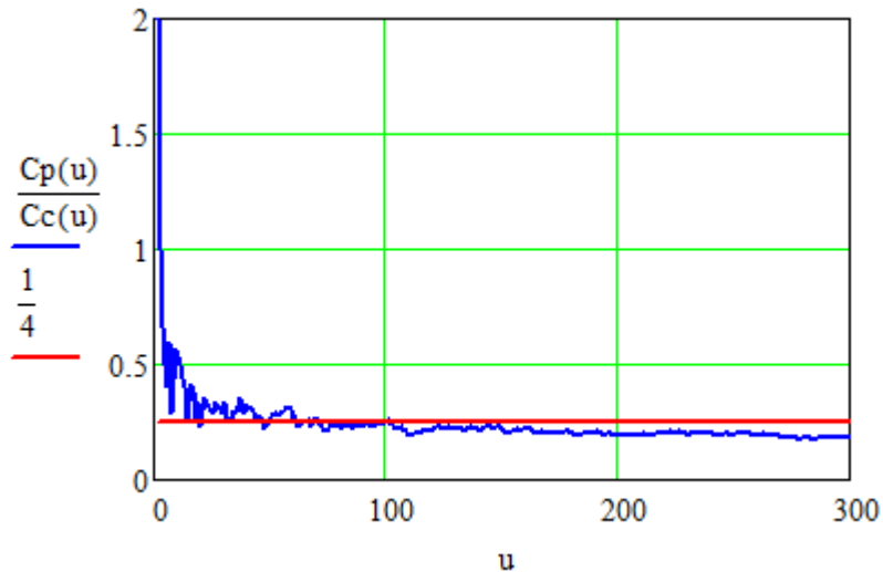
Fig. 7 Plot of the quotient C_p/C_c of the two Bertrand probabilities in the interval (2,300) showing its decreasing value as u gets large.
