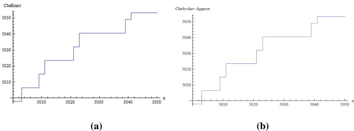
Fig. A1 Comparison plots of the exact Chebyshev function (a) in Eq. (30), and of our approximant Chebyshev Aprox (b) , in Eq. (31), in the interval [5000, 5050] with relative accuracy of order of 10^{-13} .
