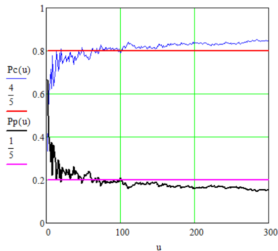
Fig. 6 Plot of the Bertrand probabilities P_p, P_c for u in the interval (2, 300) . It shows that the probability P_p for finding primes in the interval (u, 2u) decreases below 1/5 as u grows large.
