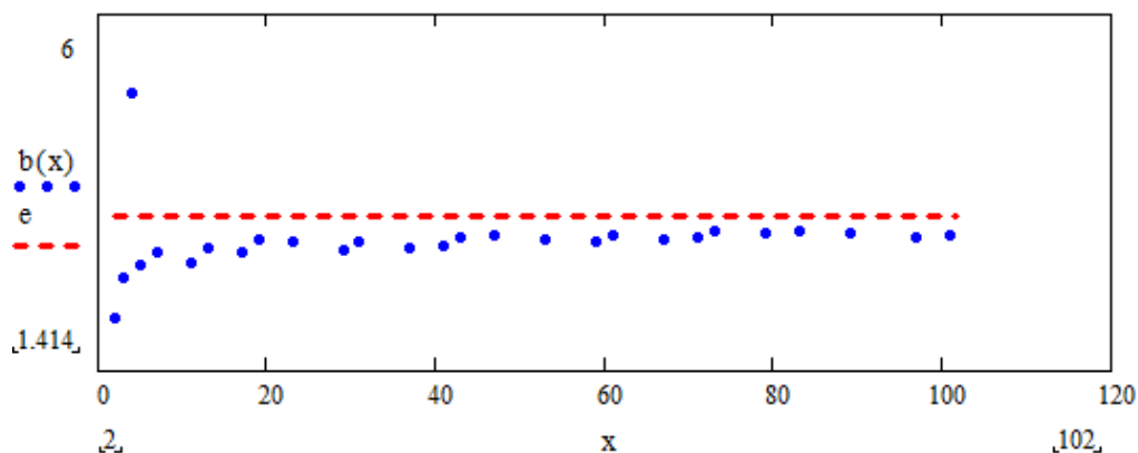
Fig. 17 Plot of the function b(x) (blue dots) showing its asymptotic limit at the constant e (red dashes)
