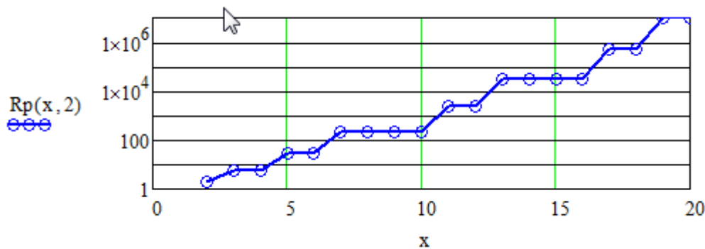
Fig. 11 Product of the prime numbers in the integer interval (2, x) up to x=20
