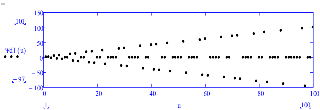
Fig. 3 Plot of the first discrete derivative of our prime numbers generating function \Psi in the integer domain [1, 100] .
