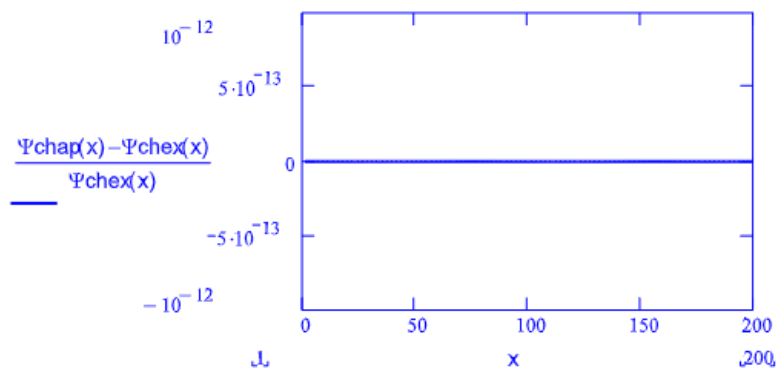
Fig. 15 Relative error (order of 10^{-13} ) of our approximant to the Chebyshev function, w.r.t. the exact function, in the interval [0,200] showing the high accuracy, of our approximant, Eq. (31) that does not use tables of primes..
