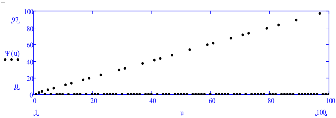
Fig. 2(a) Plot of the prime numbers in the integer interval (0, 100) given by our prime number generating function \Psi : as expected there are 25 dots lying on the inclined line.
