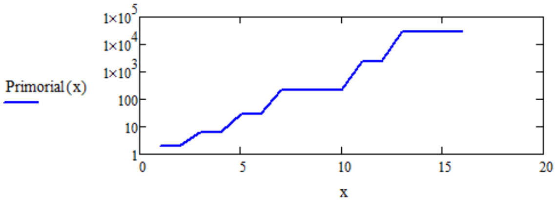
Fig. 16 Plot of the Primorial(x) function in the interval of integers (2-20), the plateau heights are explained in the text.
