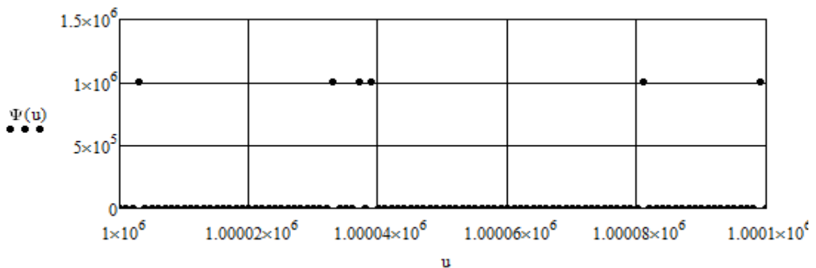
Fig. 2 (b) Plot of the six prime numbers that belong in the integer interval (1000000, 1000100) as given by the prime generating function \Psi . The dots along the abscissa axis correspond to the composite integers in that interval.
