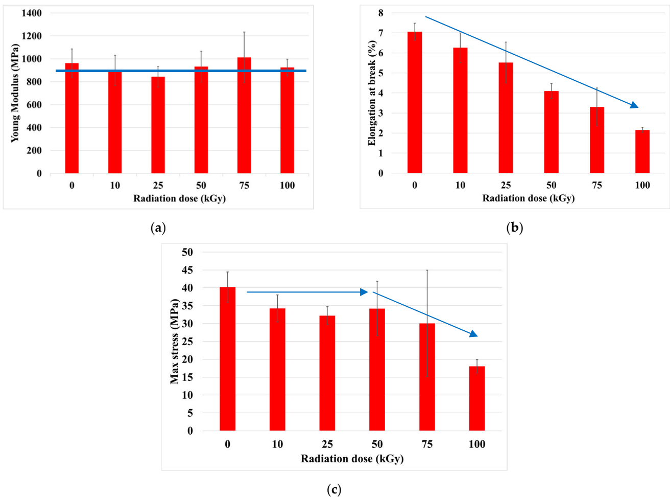
Figure 4. Influence of EB radiation dose on 3D-printed PLA specimens: (a) Young’s modulus, (b) elongation at break, (c) max stress.
