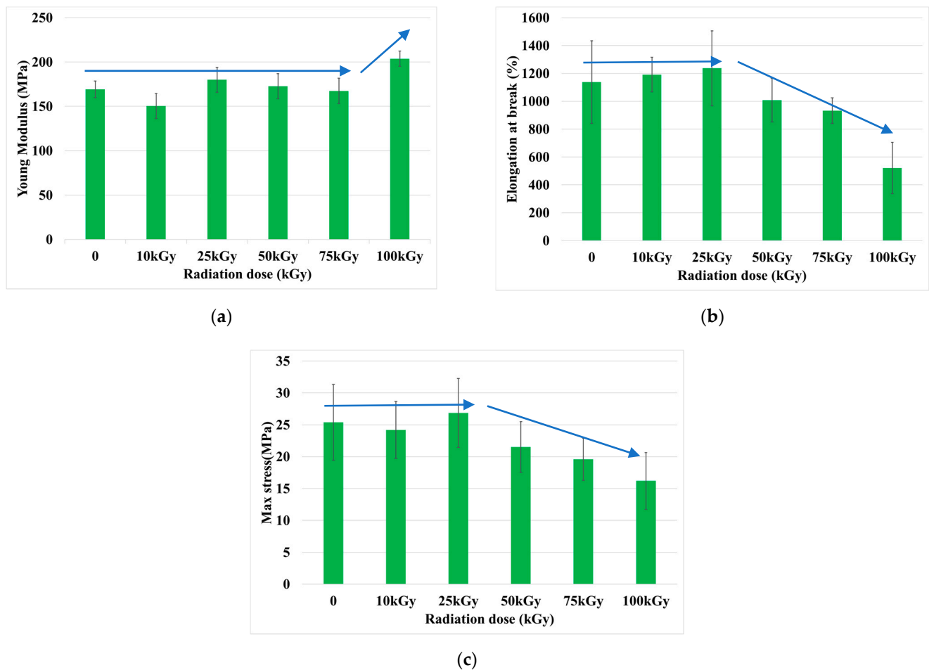
Figure 5. Influence of EB radiation dose on 3D-printed PCL specimens: (a) Young's Modulus, (b) elongation at break, (c) max stress.
