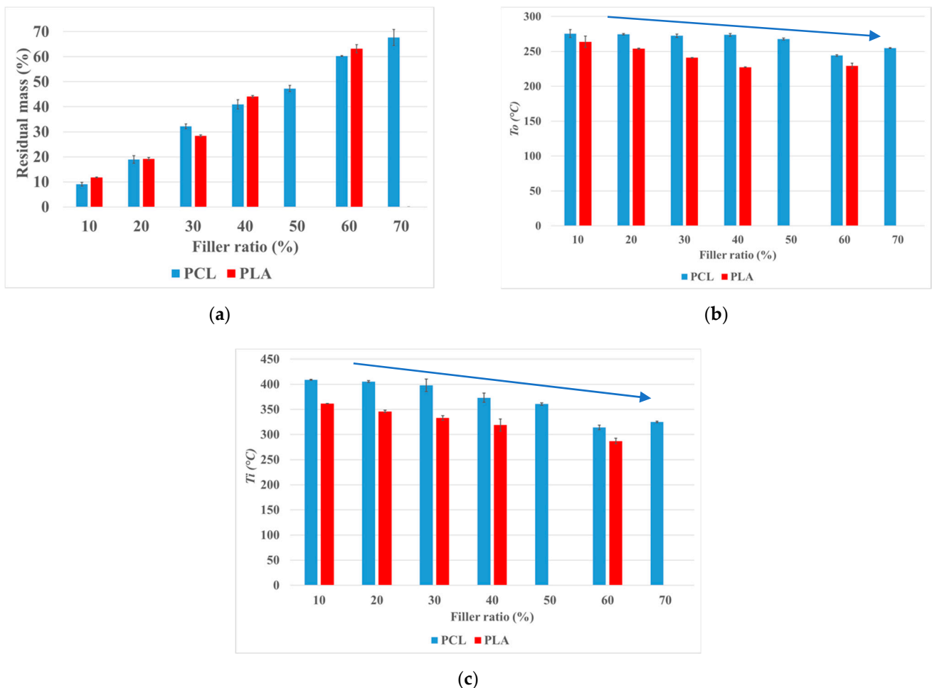
Figure 6. (a) Evaluation of mass residual in biocomposites. (b) Influence of ratio filler dose on the onset thermal degradation temperature T_0 . (c) Influence of ratio filler on the temperature of the inflection point of the degradation curve T_i .
