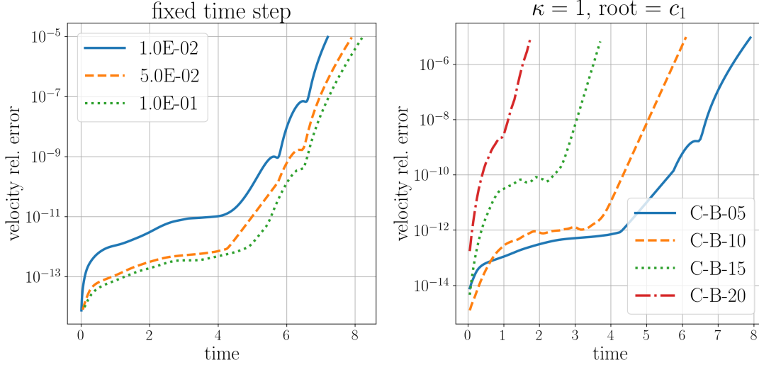
Figure 9: The effect of different time-steps (left) and orders in the B-Spline cascade interpolation (right). Larger time-steps and lower interpolation orders yield the best results. The run-time parameters are as in Figure 8.
