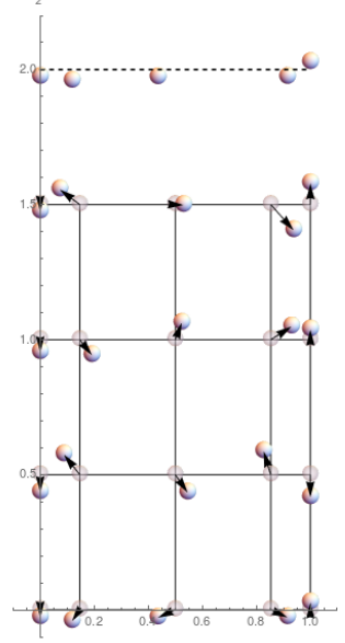
(b) Particle displacement on the (r, z) -plane on a 5 \times 4 grid. The upper row of particles have been added by periodicity.
