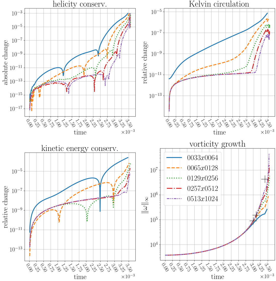
Figure 13: Resolution study with fixed parameters: S = 15 , \Delta t = 10^{-5} , Bessel-Chebyshev solver, 5th order B-spline interpolation method. The legend in the vorticity growth plots applies to all other panels. Here and in the following plots, the black crosses in the vorticity plot are the exact coordinates from Table 1 at times t = 0.003 , t = 0.0031 and t = 0.0034 . Also the helicity panel displays absolute errors, because the initial helicity vanishes for this flow.
