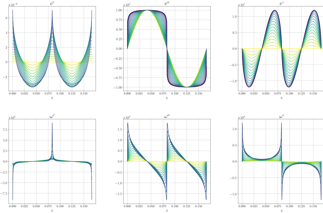
Figure 18: Upper row: Plot of the velocity components at r = 1 until t = 3.51 \times 10^{-3} . The values were obtained from a simulation with 513 \times 4096 grid points, the other run time parameters were the same as in the preceding figures. The velocity component v^r in the top left panel should stay zero at r = 1 due to the no-flow boundary condition, but large errors appear eventually at the symmetry axes. Lower row: Plot of the vorticity components at r = 1 . Here, the evolution of the components is only displayed until t = 3.0 \times 10^{-3} , the growth of the local extrema is too strong to be conveniently visualized. For surface plots of the flow field components, we would like to refer the reader to [35].
