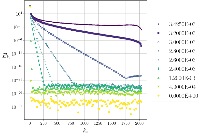
Figure 16: Energy spectrum at the boundary r = 1 for various time instances. Small modes fill up rapidly and the flow can soon not be resolved accurately anymore. The underlying grid size was fixed to 513 \times 4096 Chebyshev-Fourier points. All other fixed run time parameters are given in the text.
