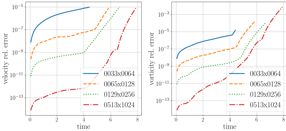
Figure 8: A visualization of relative errors in the velocity (left) and vorticity (right) fields due to different resolutions. The fixed run-time parameters are: S = 25 , time-step 0.05, 5-th order B-spline cascade interpolation.
