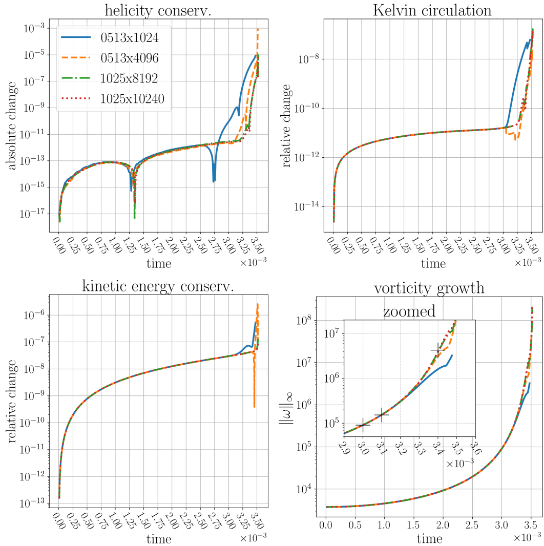
Figure 17: Higher resolution runs are shown. Here, the truncation order was set to S = 18 to maintain the initial time-step 10^{-5} longer. The interpolation was done by the 5th order B-spline cascade; no dealiasing is used here. Sudden breaks in the conserved quantities arrive much later than in the previous plots, indicating a lasting stability with increased resolution.
