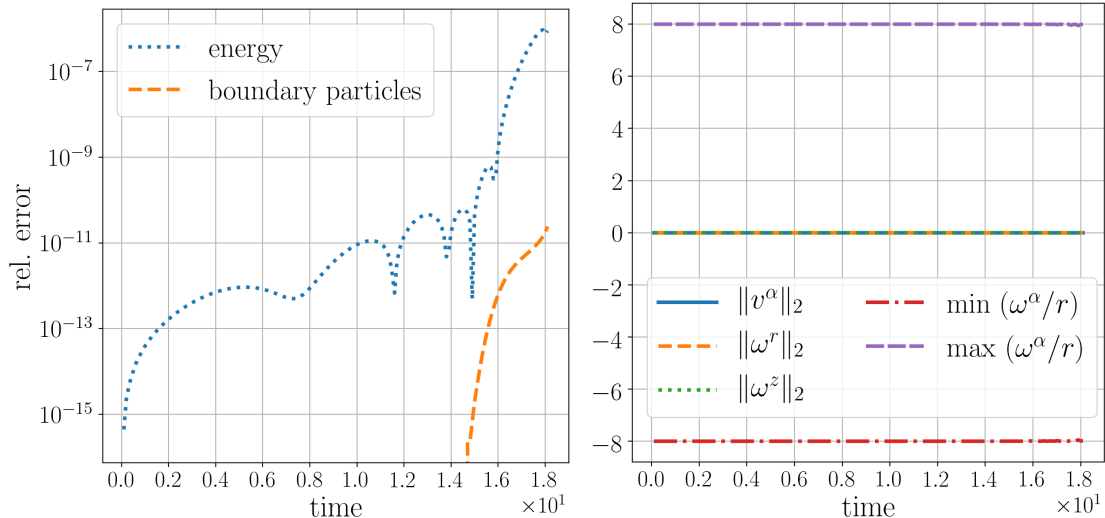
Figure 12: Test results for the given swirl-free flow with a = 1 and n = 2 , and run-time parameters: S = 20 , \Delta t = 0.1 , Chebyshev-Galerkin solver, 5th order B-spline cascade interpolation, no dealiasing, on a 513 \times 1024 Chebyshev-Fourier grid. Left: kinetic energy conservation and movement of the boundary particles in radial direction, all the conserved quantities, which are not plotted here, stayed identically zero in the simulation; Right: verification of the min/max principle for \omega^\alpha/r|_{r \neq 0} , and verification of eq. (160).
