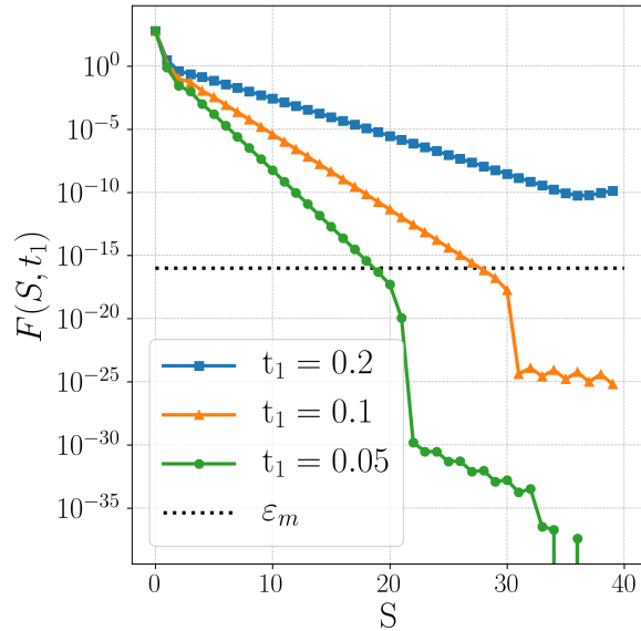
Figure 5: Plot of the function F defined in (142) for different time-steps. The recursion mechanism may be stopped, when the values of F drop below machine epsilon \varepsilon_m , here in double precision and indicated by a dotted line in the plot. All higher order terms X^{(s)} after the criterion has been met give the same summation result in the time-Taylor series in the working precision. A break in the linear behavior of F indicates the depletion of the number range in double precision in the coefficients X^{(s)} .
