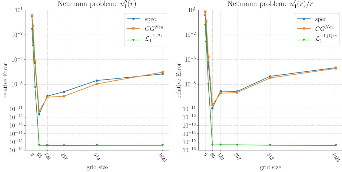
Figure 1: Convergence and accuracy verification for the methods \mathcal{L}_1^{-1,(2)} and \mathcal{L}_1^{-1,(1)/r} with the test function u_1(r) = e^{1-\cos(2\pi r)} - 1 . The RHS function is analytically calculated as f_1(r) = \mathcal{L}_1 u_1(r) and implemented exactly, the relative errors are computed in the l^2 -norm on the fixed grid. The legend references the graphs by the method that was used to obtain them. Here, the CG^{Neu} method was used to solve \mathcal{L}_1 u_1 = f_1 for the solution itself, to which standard spectral differentiation and division methods (see Section A) were applied. Those spectral differentiation and division methods, applied directly to the implemented function u_1 (no solving is involved, u_1 is directly projected into the finite dimensional Chebyshev-Fourier space), are referenced with spec.
