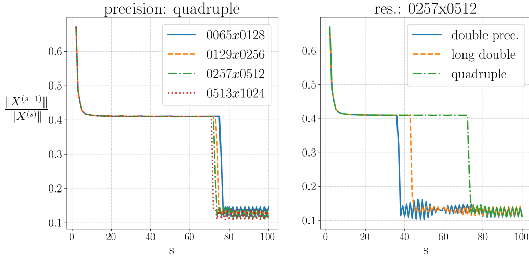
Figure 4: Approximation of the limit in eq. (139) in the l^\infty -norm on the underlying grid. The curves overlap to at least s = 30 , from which a possible limit at around 0.4 can be inferred. The sudden drop in values indicates that the working precision is insufficient to accurately represent the time-Taylor coefficients.
