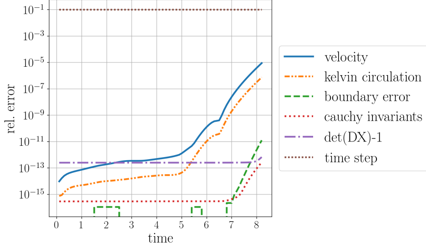
Figure 11: Test flow and conserved quantities that are particular to the CLA; same run-time parameters as in Figure 10.
