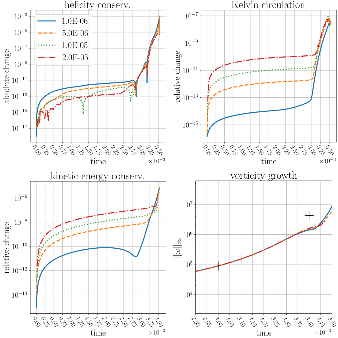
Figure 14: Several fixed time-steps are compared on a 513 \times 1024 grid; same run-time parameters, other than time-step, as in Figure 13. Larger time-steps deliver good and fast results. The legend in the first panel is valid for the others too. Note that the fourth panel does not show the whole integration period.
