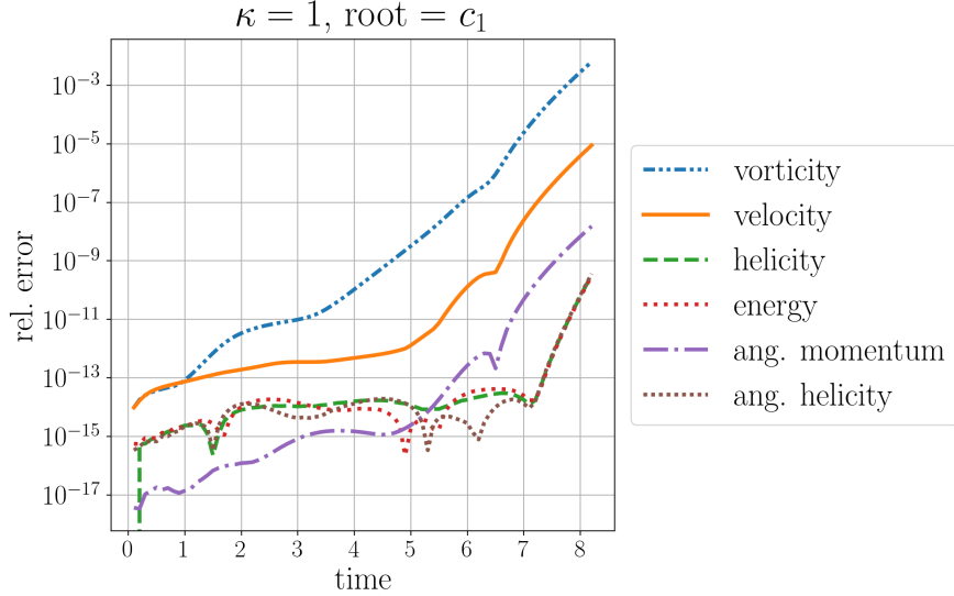
Figure 10: Test flow and standard conserved quantities, computed on 513 \times 1024 points, with S = 40 , time-step \Delta t = 0.1 , Chebyshev-Galerkin solver and 5th order B-spline cascade interpolation.
