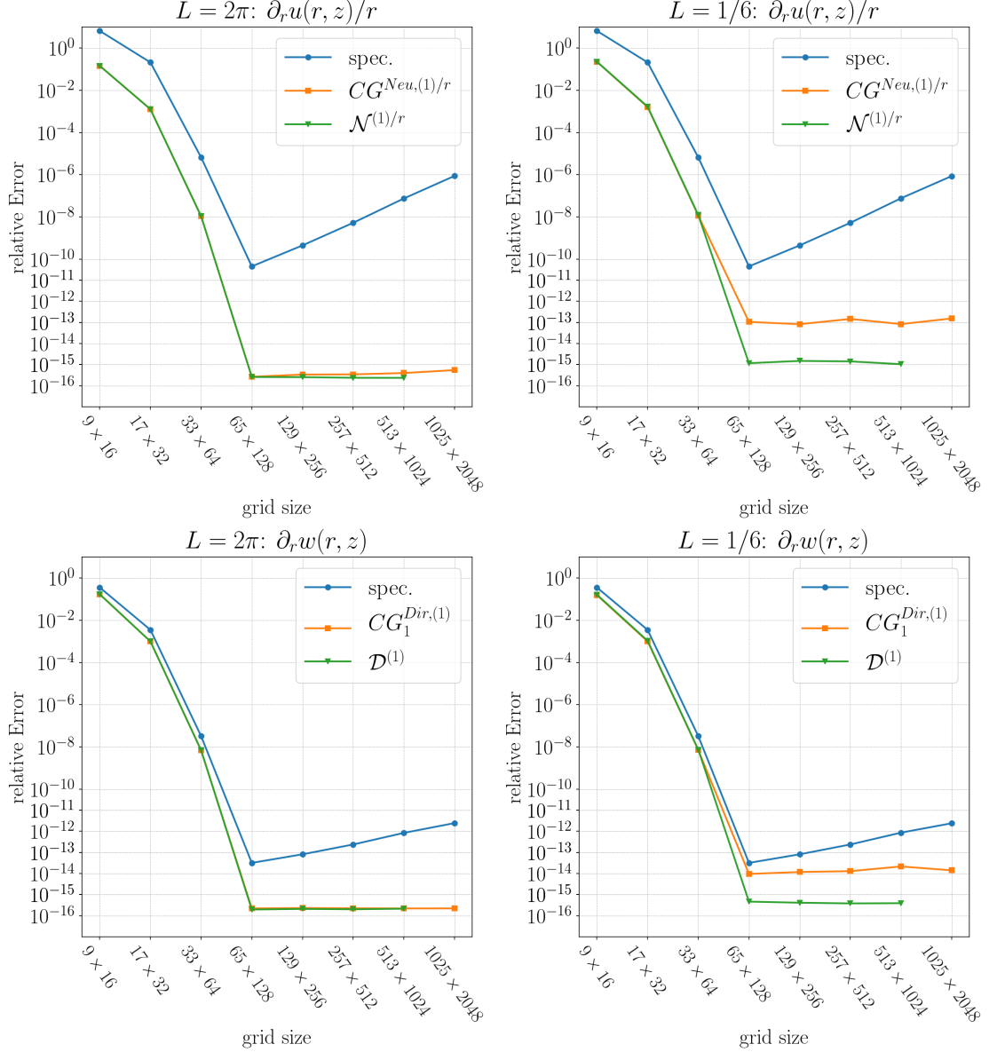
Figure 2: Derivative of the approximated solution to eq. (64) divided by r and derivative of the approximated solution to eq. (65) for L = 2\pi and L = 1/6 . The analytic solutions are u(r, z) = w(r, z) = u_1(r) e^{\sin(2\pi z/L)} , with u_1 as in Figure 1. The relative errors are computed with the l^2 -norm on the fixed Chebyshev-Fourier grid.
