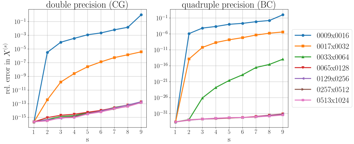
Figure 7: Relative errors (as defined in (158)) in the computed coefficients X^{(1)}, \dots, X^{(9)} , which belong to the flow in eq. (156) with \kappa = 1 and c_1 . The Poisson problems were solved in double precision via the Chebyshev-Galerkin solver (left) and in quadruple precision via the Bessel-Chebyshev solver (right). The true coefficients were obtained via symbolic differentiation inside a computer algebra system by the method described in Section B.
