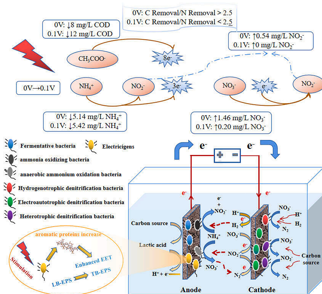
Fig. 6. Demonstration of denitrification pathway under function of MUIWES.
