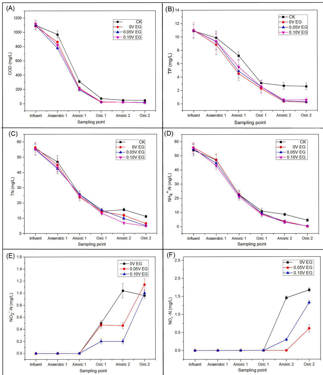
Fig. 3. (A) COD, (B) TP, (C) TN, (D) NH 4 + -N, (E) nitrite (NO 2 - -N) and (F) nitrate (NO 3 - -N) in the successive treatment steps of the A-(A/O) 2 system equipped with a MFC providing MUIWES to a MEC. CK: control without MFC and MEC. Voltage refers to voltage applied to the MEC.
