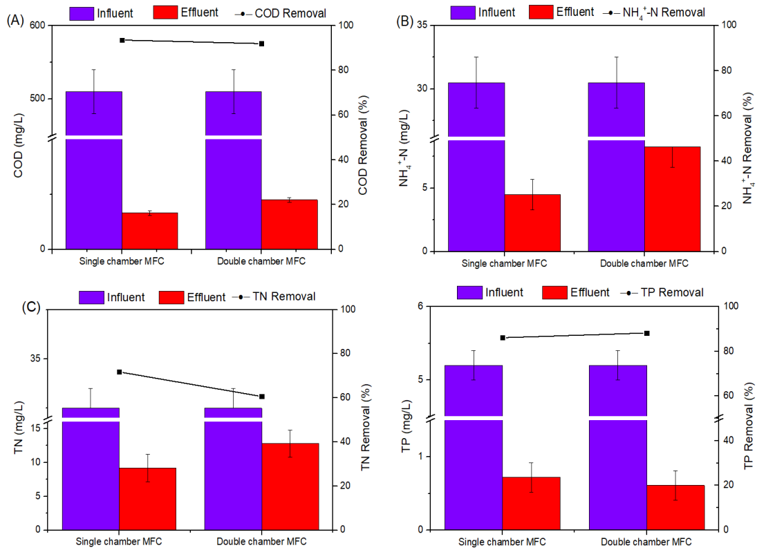
Supplementary Figure S3 Total removal in mg/L and percentage of the COD (A), NH 4 + -N (B), TN (C) and TP (D) in the A-(A/O) 2 system equipped with different anode MFCs
