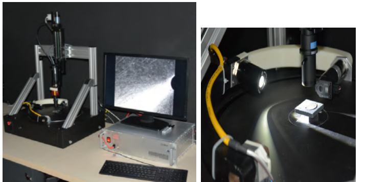
Fig. 2. Home-made x-RTI system for surface appearance acquisition.
