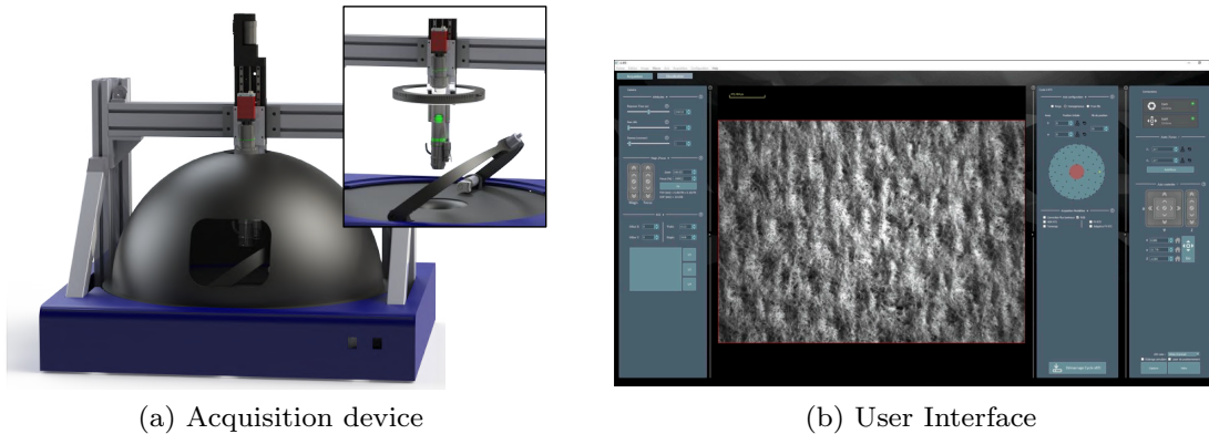
(a) Acquisition device (b) User Interface Figure 3. Custom RTI acquisition system (ImViA Laboratory), from . 12
