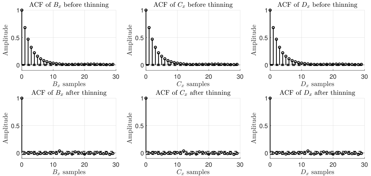
Figure 21: Autocorrelation functions of a Markov chain when the friction measurements are lower than \mu = 0.25 . The upper figures represent the ACF before thinning. The lower figures illustrate the ACF after thinning. In all figures, the dashed black lines represent the standard error of the ACF with a confidence interval of 95%.
