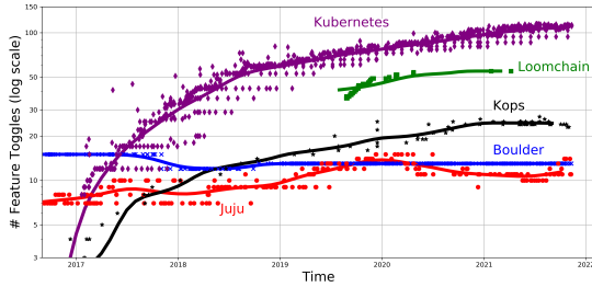
Figure 1: Evolution of feature toggles (y-axis, log scale) over time (x-axis) - Each point represents a change of toggles
