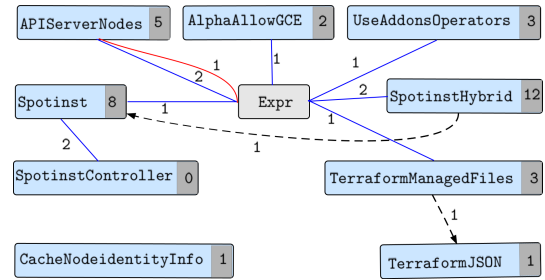
Figure 3: An excerpt from the Feature Toggle Model of Kops
