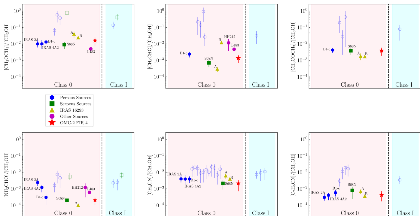
Fig. B.8. Abundance ratio of iCOMs with respect to \text{CH}_3\text{OH} in HOPS-108 compared to other isolated hot corinos. The sources are separated according to their class, with no particular order within a given class. The open symbols correspond to the sources where the \text{CH}_3\text{OH} column density is most likely underestimated due to its high optical depth (See Sect. 4.2.1). The Class 0 sources are: IRAS 2A, IRAS 4A2 (Taquet et al. 2015; López-Sepulcre et al. 2017), B1-c, S68N (van Gelder et al. 2020; Nazari et al. 2021), IRAS19347 + 0727 in B335 (Imai et al. 2016), HH212 (Bianchi et al. 2017; Lee et al. 2019), L483 (Jacobsen et al. 2019), Ser-emb 1 (Bergner et al. 2019), IRAS 16293 A (Manigand et al. 2020; Calcutt et al. 2018), IRAS 16293 B (Jørgensen et al. 2016, 2018; Lykke et al. 2017; Calcutt et al. 2018), HOPS-108 in OMC-2 FIR 4 (this work), and the sources from the PEACHES survey (Yang et al. 2021), including Per-emb 1, Per-emb 2, Per-emb 5, Per-emb 10, Per-emb 11A, Per-emb 11C, Per-emb 12, Per-emb 13, Per-emb 18, Per-emb 20, Per-emb 21, Per-emb 22A, Per-emb 22B, Per-emb 26, Per-emb 27, Per-emb 29, Per-emb 33A, L1448 IRS3A, L1448-NW, SVS-13B, and B1-bS. The Class I sources are: Ser-emb 17 (Bergner et al. 2019), L1551 (Bianchi et al. 2020), and also sources from the PEACHES survey (Yang et al. 2021), including Per-emb 35A, Per-emb 35B, Per-emb 42, Per-emb 44, Per-emb 53, and SVS13-A2. The same plots for \text{HCOOCH}_3 and \text{CH}_2\text{DOH} are represented in Figs. 4 and 6, respectively.
