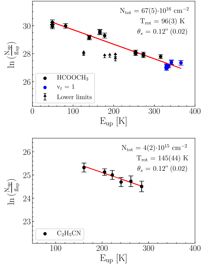
Fig. 3. Rotational diagrams for \text{HCOOCH}_3 (top) and \text{C}_2\text{H}_5\text{CN} (bottom). Data points are presented in black. The \text{HCOOCH}_3 v_t = 1 transitions are depicted in blue. The arrow symbols represent the lower limits that are excluded from the analysis (see Sect. 3.4). The red lines correspond to the best fit to the data points.
