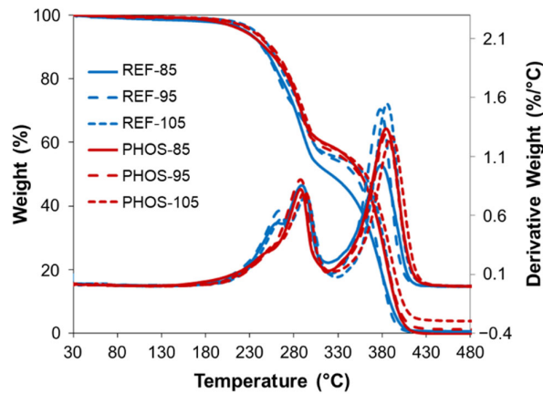
Figure 6. TGA and DTG curves of flexible foams (inert atmosphere).
