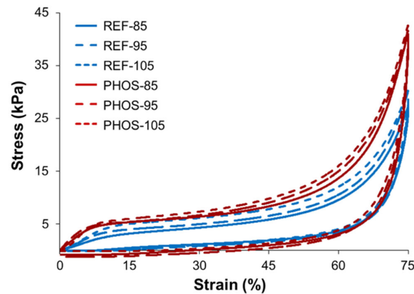
Figure 7. Hysteresis loops of flexible foams.
