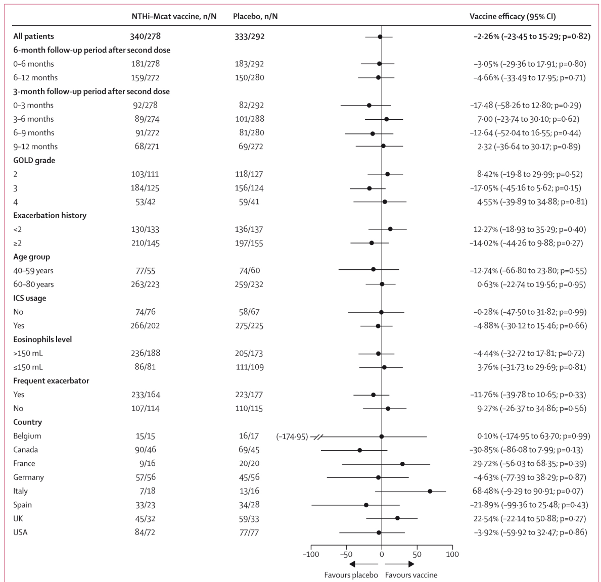
Figure 3: Forest plot of vaccine efficacy for moderate and severe AECOPD in each subgroup analysis for 1 year starting from 1 month after the second dose (modified total vaccinated cohort; n=571)
