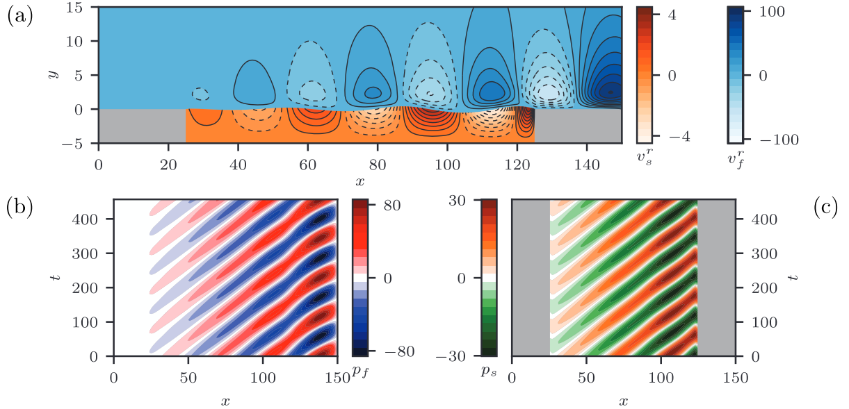
Figure 13: Perturbation field for the coupled response to the rigid, harmonic, optimal forcing at the TSW amplification peak (● in Figure 12). The blue and orange shaded contours in (a) report respectively the real part of the transverse velocity for the fluid and solid medium; dashed contours indicate negative values. (b-c) report the pressure perturbation as a function of space and time: (b) shows the response in the fluid phase at y = 1 , while (c) in the solid phase at y = -1 .
