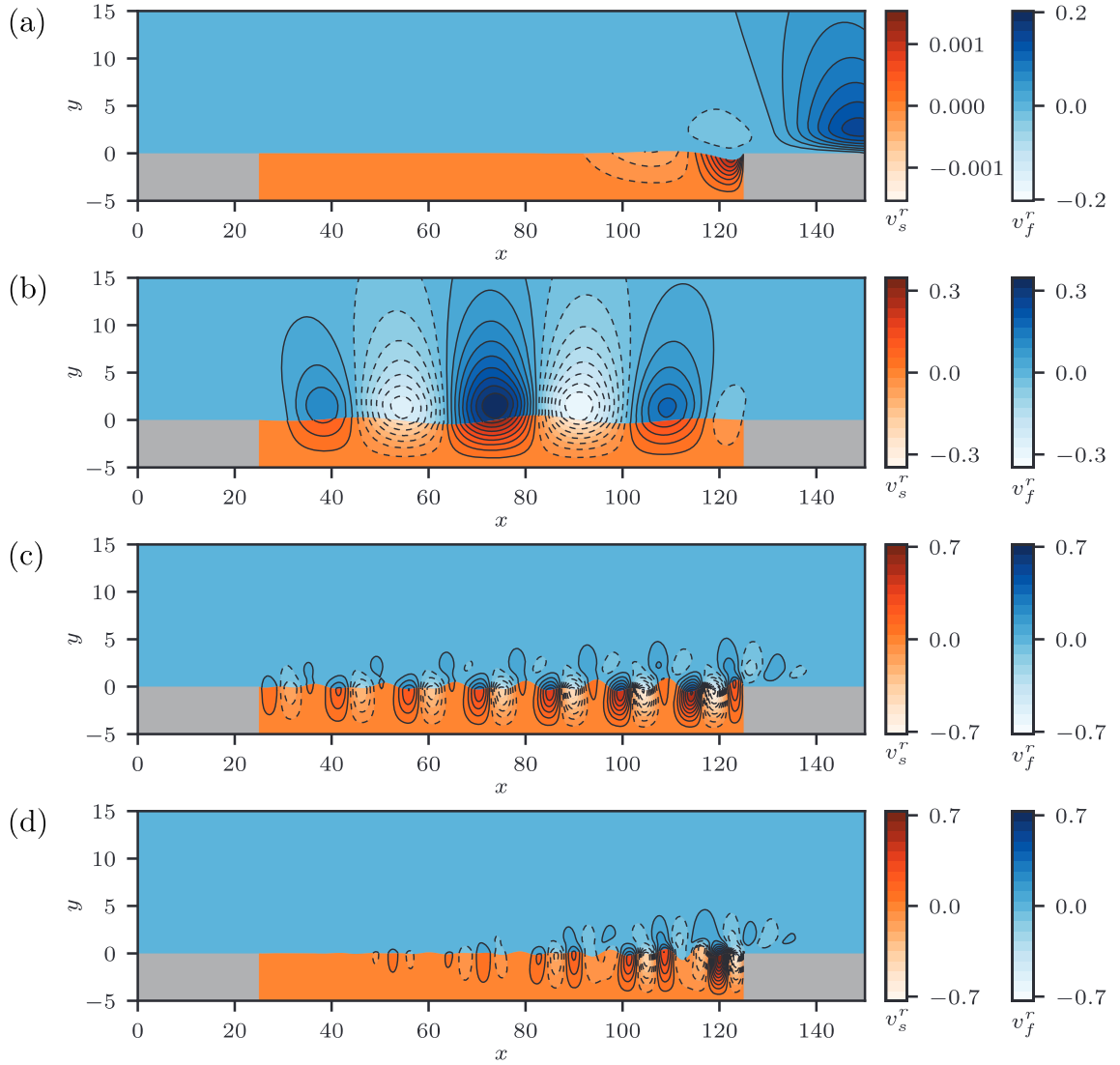
Figure 7: Modes shapes corresponding to the eigenvalues labelled (a)–(d) in Figure 6. Dashed contours indicate negative values.
