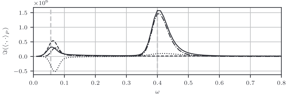
Figure 21: Production decomposition according to Equation 5.6. The production term for the coupled optimal response ( \langle \mathbf{q}_f, \mathbf{q}_f \rangle_P , solid line —) is decomposed in the contributions of the rigid-wall response ( \langle \hat{\mathbf{q}}_f, \hat{\mathbf{q}}_f \rangle_P , dashed line ---), the feedback fluid-solid response ( \langle \mathbf{r}_f, \mathbf{r}_f \rangle_P , dot-dashed line -.-), and the cross-product term ( \langle \mathbf{r}_f, \hat{\mathbf{q}}_f \rangle_P + \text{c.c.} , dotted line .....). The dashed grey vertical lines indicate the frequencies for which the decomposed responses are reported in Figure 23 and Figure 24.
