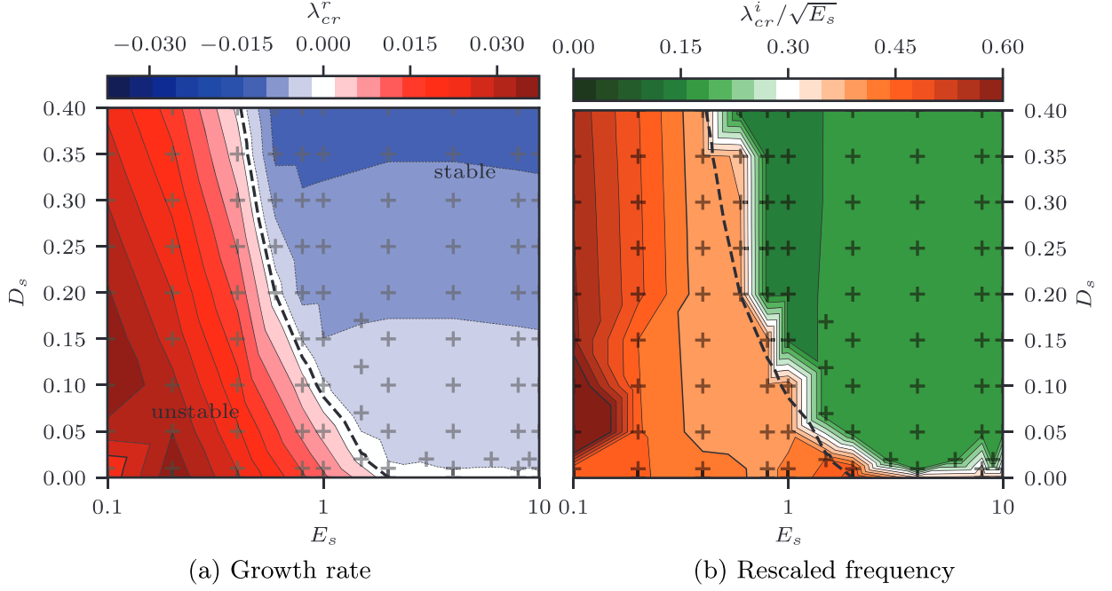
Figure 9: Influence of the viscoelastic damping D_s and stiffness E_s on the fully coupled fluid-solid spectrum. (a) reports the real part of the most unstable eigenvalue \lambda_{cr} , while (b) its rescaled imaginary part: the dashed lines separate the stable and unstable regions of the parameters' space. The imaginary part has been scaled with the solid quantities, i.e. by the square-root of the Young's modulus E_s . The crosses indicate the combinations of (E_s, D_s) for which the spectrum has been computed.
