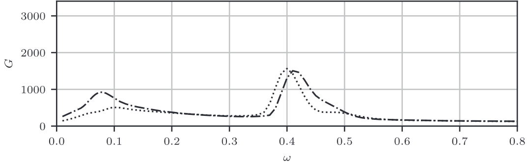
Figure 15: Coupled response ( E_s = 1 and D_s = 0.2 ) to the the sub-optimal, rigid forcings. The energetic amplification ( G ) to the first and second suboptimals are reported by the dot-dashed (---) and dotted (.....) lines, respectively.
