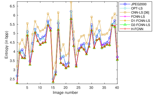
Fig. 8. Entropy values for the different images of the CLIC dataset.
