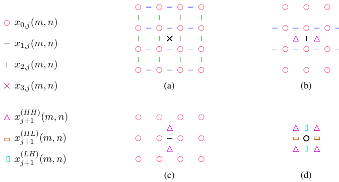
Fig. 7. Spatial supports of the prediction and update filters used to generate: (a) the diagonal detail coefficients x_{j+1}^{(HH)} , (b) the vertical detail coefficients x_{j+1}^{(HL)} , (c) the horizontal detail coefficients x_{j+1}^{(LH)} , and (d) the approximation coefficients x_{j+1} . Note that for every step, the pixels to be predicted and updated are highlighted in black.
