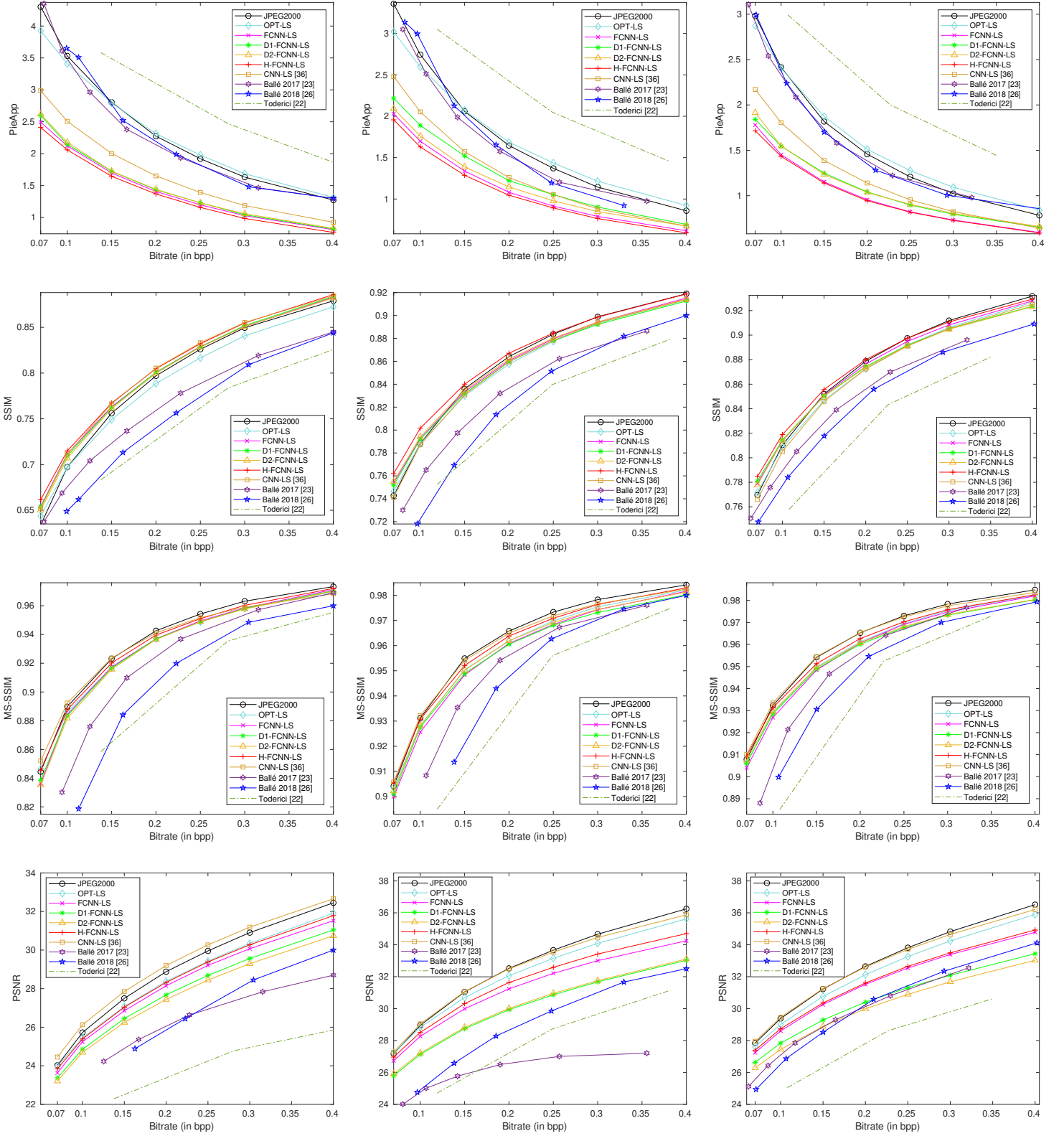
Fig. 10. Average R-D results of the CLIC (first column), Tecnick-R1 (second column) and Tecnick-R2 (third column) image datasets using PieAPP, SSIM, MS-SSIM and PSNR metrics.
