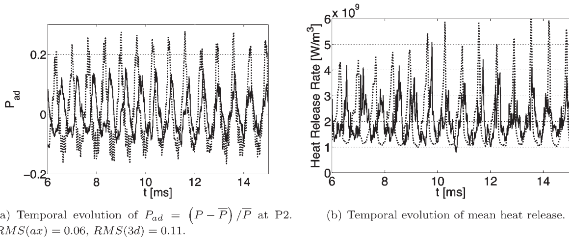
Fig. 8. --- 3D, — axis-symmetric.
