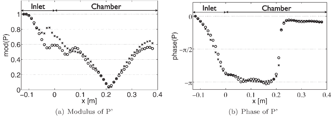
Fig. 9. Structure of the acoustic field, \times : 3D, \circ : 2D axis-symmetric.
