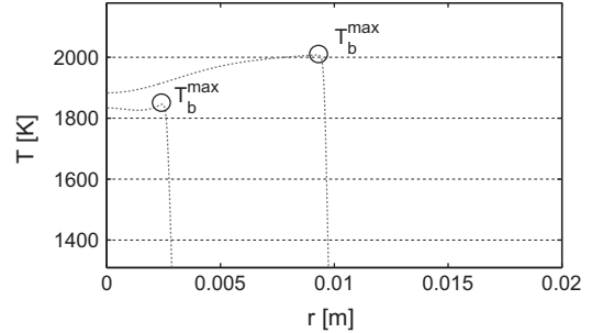
Fig. 5. Definition of T_b^{\max} with the temperature profiles vs. the flame radius r .
