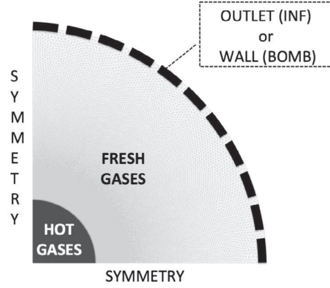
(b) Computational domain for the cylindrical flame.
