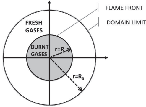
(a) Generic configuration for a spherical flame in a bomb.
