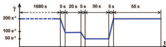
Fig. 2. Example of a time sequence for a three-point rheogram.
