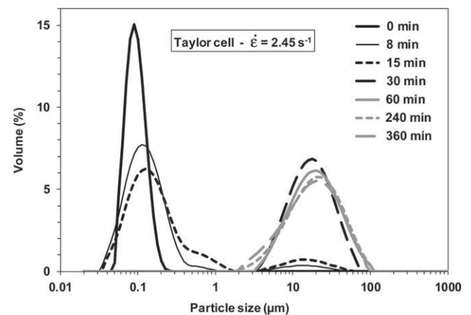
Fig. 10. Volumetric PSD of the suspension in the Taylor cell for an extensional rate \dot{\epsilon} = 2.45 \text{ s}^{-1} .
