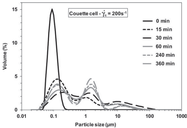
Fig. 8. Volumetric PSD of the suspension in the Couette cell for a shear rate \dot{\gamma}_c = 200 \text{ s}^{-1} .
