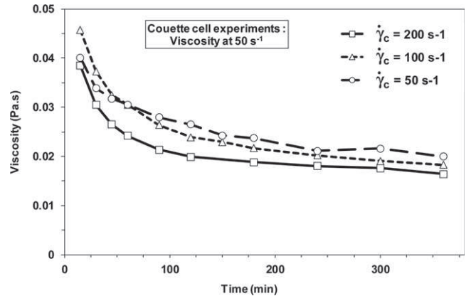
Fig. 6. Viscosity of the suspension in the Couette cell at 50 \text{ s}^{-1} for the three experimented main shear rate \dot{\gamma}_c .
