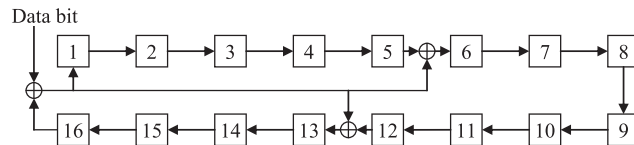
Figure 2. Example of iterative cyclic redundancy check computation with the generator polynomial G(x) = x^{16} + x^{12} + x^5 + 1 . \oplus represent XOR and are placed according to the generator polynomial. The numbered boxes contain the derived cyclic redundancy check bits.
