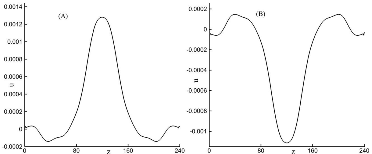
Fig. 18. Transverse profile of the velocity u along the mid z axis (at x = L/2, y = W/2 ) and at t = 600 (A) and 1100 (B).
