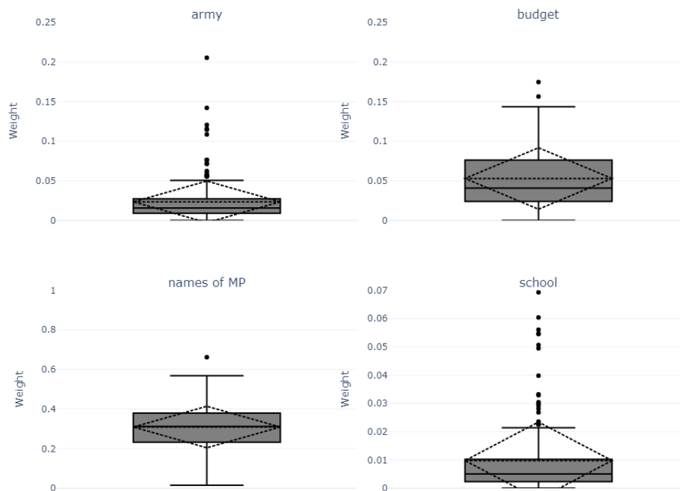
Figure 1: Comparative variances of several topic classes
