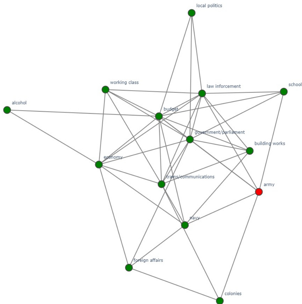
Figure 6: Graph of topics with high correlation
