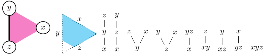
FIGURE 2. The hypergraph, the truncated simplex and the constructs associated with the hypercube \mathbf{C}
