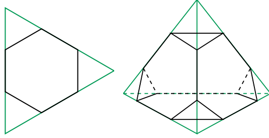
FIGURE 4. Erosohedra in dimension 2 and 3
