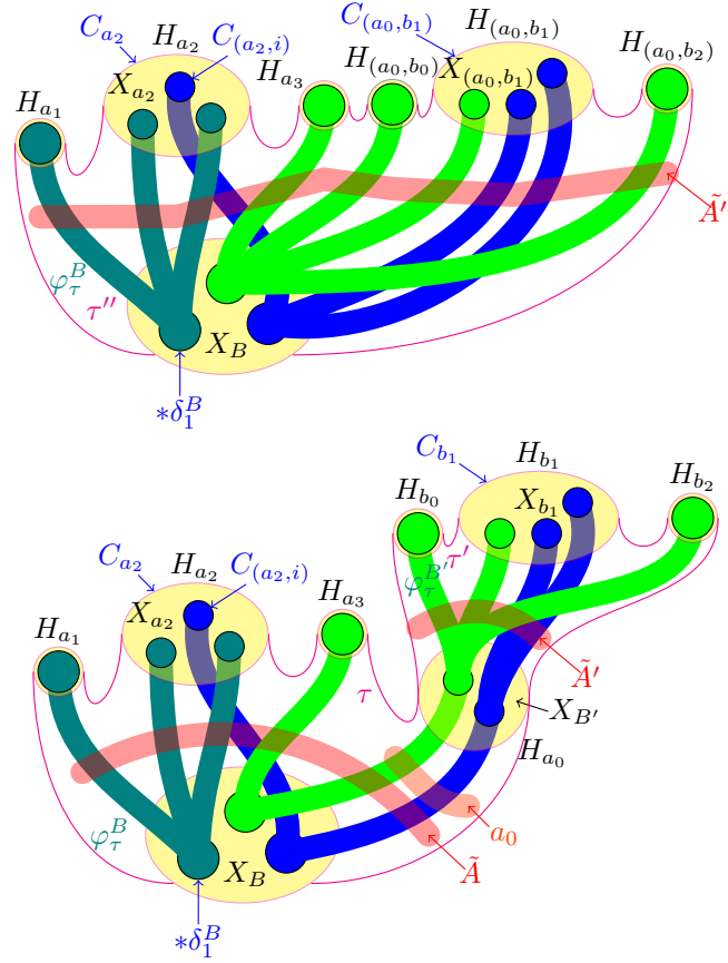
FIGURE 8. Illustration of associativity via cobordisms. We have: A = \{a_0, \dots, a_3\} , A' = \{b_0, \dots, b_2\} , A'' = \{a_1, \dots, a_3, (a_0, b_0), (a_0, b_1), (a_0, b_2)\} , B'' = \{a_2, (a_0, b_1)\} , B' = b_1 and B = a_2, a_0 .
