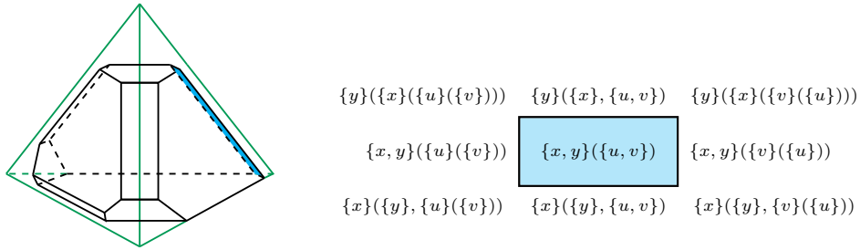
FIGURE 3. A truncated simplex
