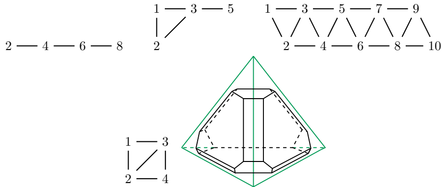
FIGURE 5. Top: Examples of friezohedra. The rightmost one is the (compact) friezohedron on \{1, \dots, 10\} Bottom: Hypergraph and truncated simplex associated with the compact friezohedron on 4 vertices
