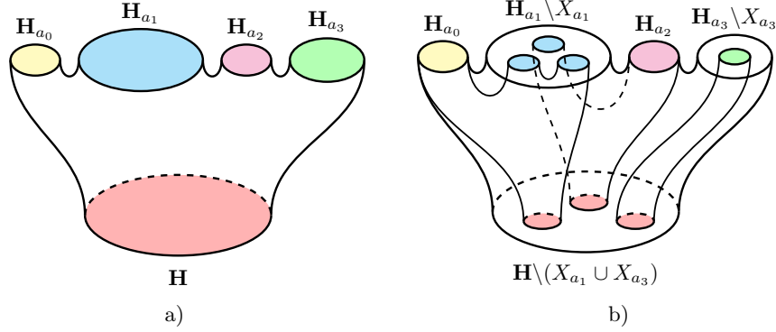
FIGURE 7. a) A preteam \tau = (\{\mathbf{H}_{a_0}, \mathbf{H}_{a_1}, \mathbf{H}_{a_2}, \mathbf{H}_{a_3}\}, \mathbf{H}) is represented as a cobordism whose upper and lower boundary disks feature the participating and coordinating hypergraphs, respectively. b) For X_{a_1} \subseteq H_{a_1} and X_{a_3} \subseteq H_{a_3} , the decompositions \mathbf{H}_{a_1} \setminus X_{a_1} \rightsquigarrow \mathbf{H}_{(a_1,1)}, \mathbf{H}_{(a_1,2)}, \mathbf{H}_{(a_1,3)} , \mathbf{H}_{a_3} \setminus X_{a_3} \rightsquigarrow \mathbf{H}_{(a_3,1)} and \mathbf{H} \setminus (X_{a_1} \cup X_{a_3}) \rightsquigarrow \mathbf{H}_1, \mathbf{H}_2, \mathbf{H}_3 are represented by “embeddings of little disks into big disks”, in such a way that the little disks represent the corresponding connected components, and their complements in big disks are the removed sets. This allows us to visualize the induced preteams \tau, X_{a_1} \cup X_{a_3} \rightsquigarrow \tau_1, \tau_2, \tau_3 as cobordisms in the interior of \tau .
