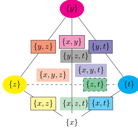
FIGURE 1. Simplex \mathbf{S}^{\{x,y,z,t\}} labeled by the subsets associated to each face. Faces of dimension k are labeled by sets of size k + 1 . We blended colors to represent inclusion of faces. The interior of the simplex is labeled by \{x, y, z, t\} .
