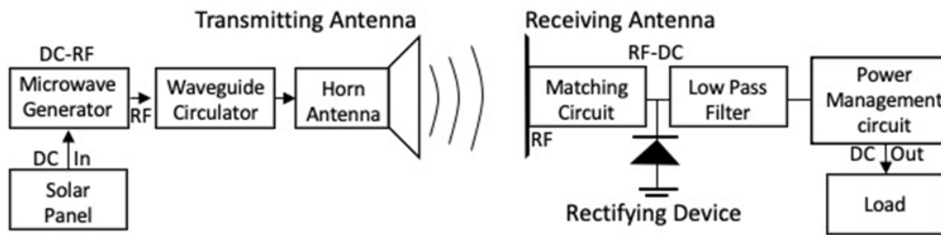
Fig. 7. Schematic Diagram of Microwave Power Transmission System.
