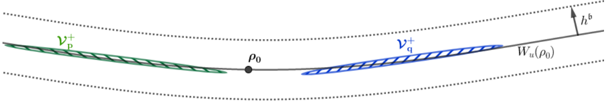
FIGURE 11. Two words \mathbf{q}, \mathbf{p} \in Q(n, a) are close to each other if \mathcal{V}_q^+ and \mathcal{V}_p^+ lie in the h^b -neighborhood of the same unstable leaves, as stated in Definition 4.1.
