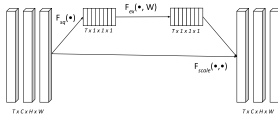
Fig. 3: Schematic diagram of SE block showcasing the squeeze and excitation function.
