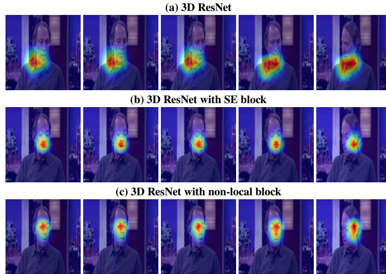
Fig. 7: Grad-CAM visualizations for the 3D ResNet models for the same video. The frames are taken from the same fake video with a time step of 24. Red represents higher probability of the region being manipulated.
