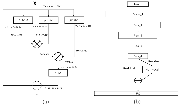
Fig. 1: Schematic diagrams of (a) non-local block, (b) non-local block in the backbone architecture.
