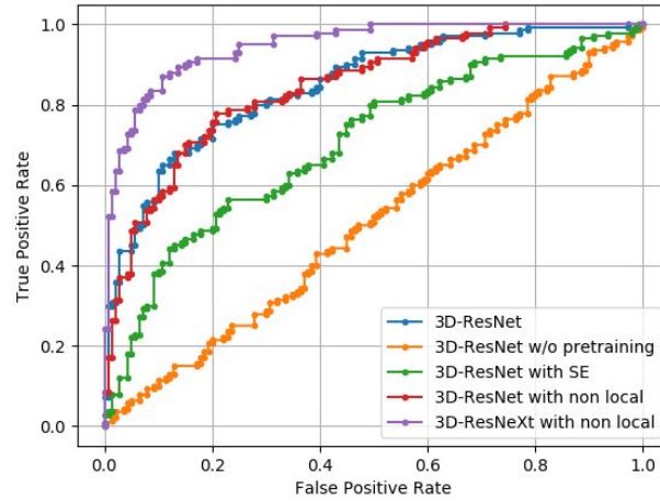
Fig. 5: ROC curves pertaining to 3D ResNet and 3D ResNext endowed with attention mechanisms for testing and training of all four manipulation methods.
