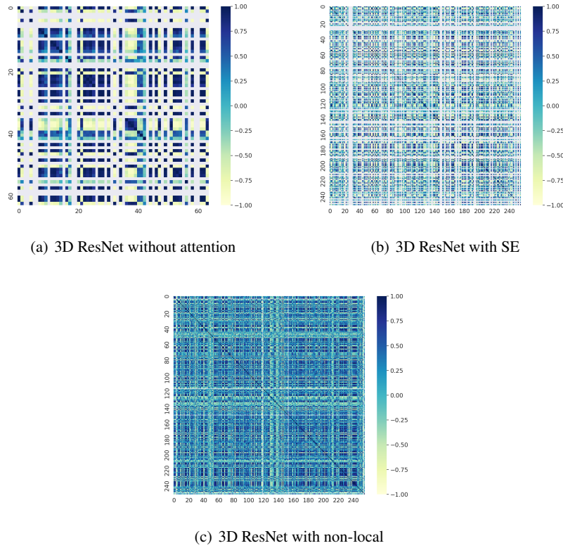
Fig. 6: Correlation matrices for the 3D ResNets
