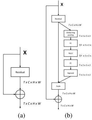
Fig. 2: (a) Residual block, (b) residual block after adding SE block.
