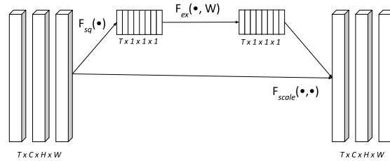
Fig. 3: Schematic diagram of SE block showcasing the squeeze and excitation function.
