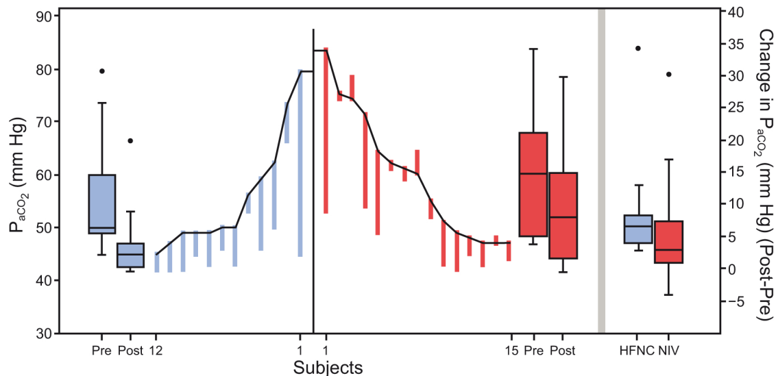
Fig. 2. P_{aCO_2} in hypercapnic subjects with cardiogenic edema receiving high-flow nasal cannula or noninvasive ventilation. Hybrid parallel line plot showing P_{aCO_2} values from baseline (pre) to after a 1-h ventilatory session (post) with HFNC (blue) or NIV (red). The lines depict change in P_{aCO_2} for each subjects, the box plot depicts median P_{aCO_2} and quartiles. Median changes in P_{aCO_2} are shown in the farther right pane. The black circle indicates outliers. HFNC = high-flow nasal cannula, NIV = noninvasive ventilation.
