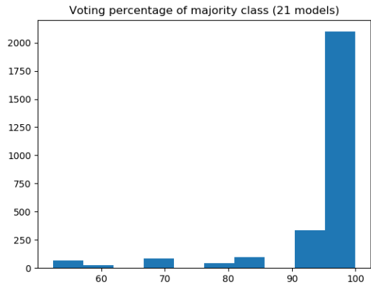
Fig. 4. Distribution of the percentages of votes given to the selected class (majority voting).
