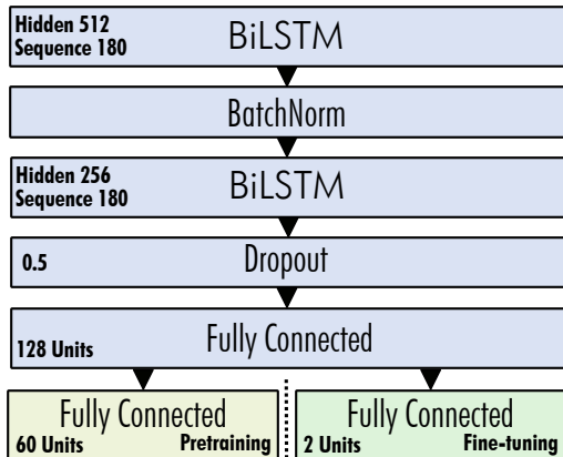
Fig. 5. Baseline BiLSTM model structure for pre-training (left) and fine-tuning on protective action prediction.
