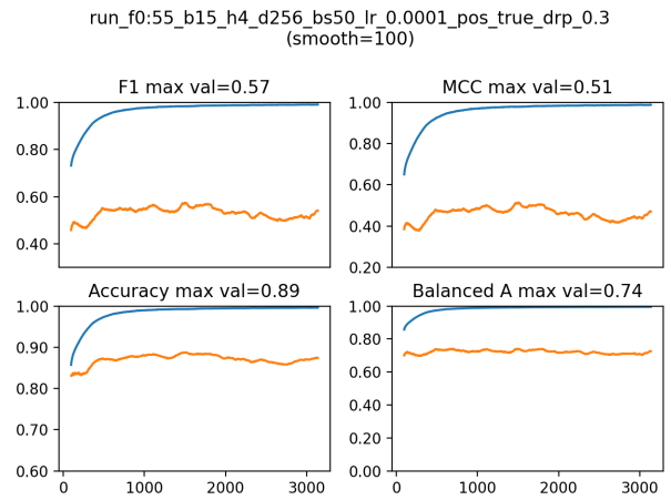
Fig. 2. Evolution of several performance metrics ( F_1 , MCC, Accuracy and Balanced Accuracy) during training for a specific tested Transformer architecture (blue training set, orange validation set) - values have been smoothed averaging the 100 surrounding values of each point. The architecture used all 55 features, 15 blocks, 4 heads, embedding sizes of 256, used positional embedding; training has been made using a batch size of 50 and a learning rate of 10^{-4} .
