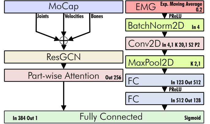
Fig. 7. Architecture of the multimodal PA-ResGCN-N51 + EMG CNN system. The final run only includes the left branch without EMG.
