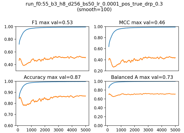
Fig. 3. Similar to Figure 2 with different hyperparameters: 55 features, 3 blocks, 8 heads, embedding sizes of 256, used positional embedding; training has been made using a batch size of 50 and a learning rate of 10^{-4} .
