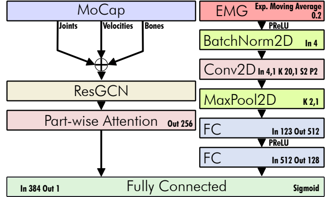
Fig. 7. Architecture of the multimodal PA-ResGCN-N51 + EMG CNN system. The final run only includes the left branch without EMG.
