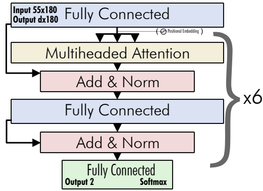
Fig. 1. The transformer baseline architecture.
