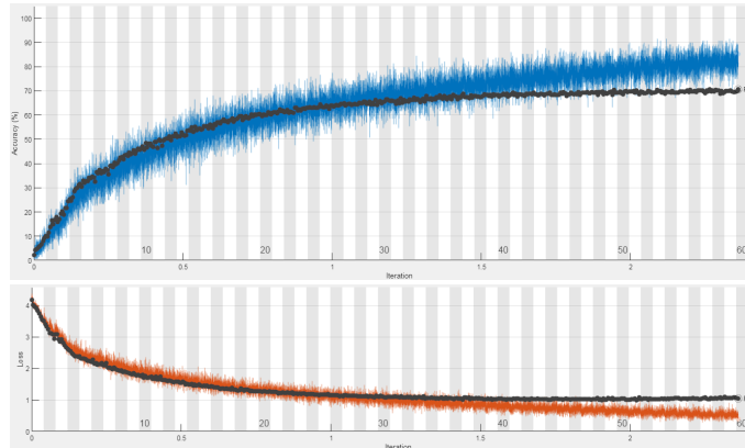
Fig. 6. Pre-training process on NTU RGB+D dataset. NTU RGB+D dataset is randomly split into training 90% and validation 10% sets in which the classes are stratified. The stopping validation accuracy at 57 epochs on the 60 classes is 70.69%.
