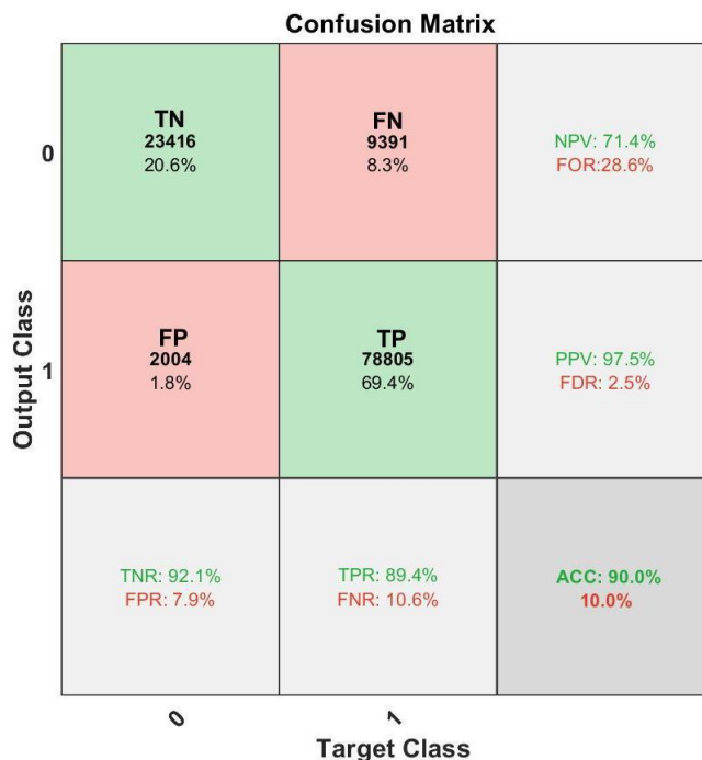
Figure 6. Confusion matrix of the performance verification with LSTM.
