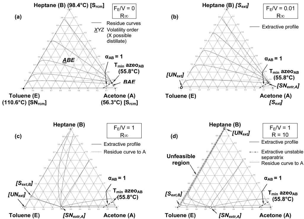
Figure 4. Separation of acetone–heptane using toluene: (a) class 1.0-1a residue curve map (rcm) and batch extractive profile map; (b) F_E/V = 0.01, R_\infty ; (c) F_E/V = 1, R_\infty ; and (d) F_E/V = 1, R = 10 .
