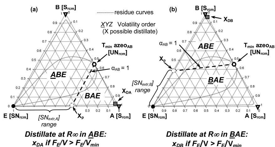
Figure 2. Thermodynamic features of class 1.0-1a mixtures with respect to batch extractive distillation: separation of a minimum-boiling azeotrope with a heavy entrainer.
