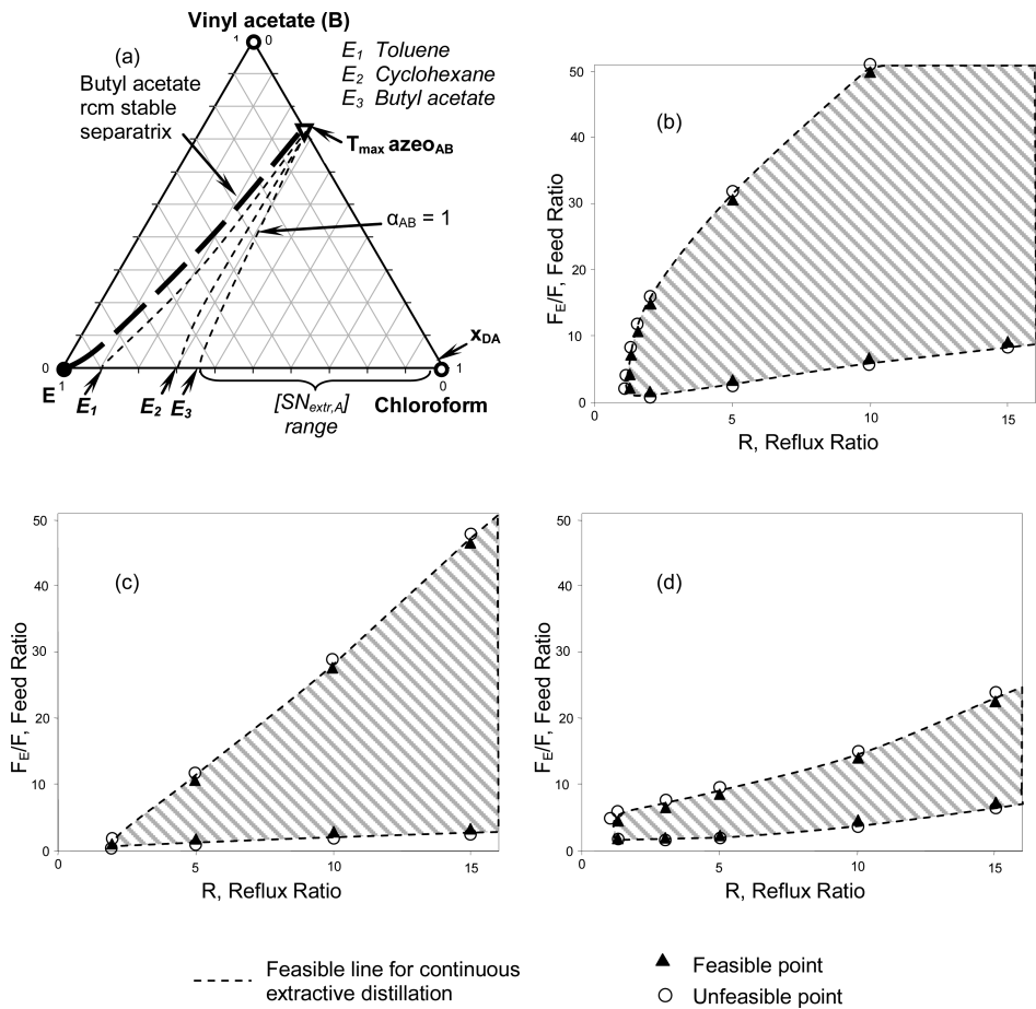
Figure 13. Comparison of three different entrainers to recover chloroform (A) from chloroform–vinyl acetate: (a) univolatility curve location and (b) toluene, (c) cyclohexane, and (d) butyl acetate feasible regions.
