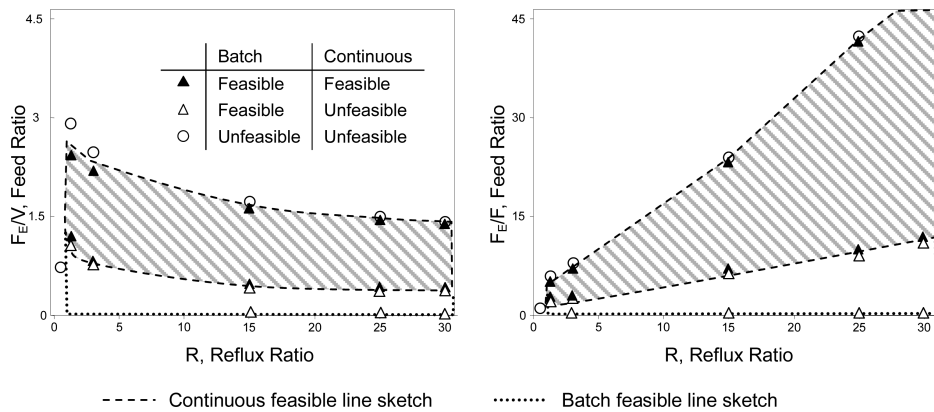
Figure 12. Feasibility of batch and continuous extractive distillation of chloroform–vinyl acetate with butyl acetate (class 1.0-2). Feed ratio as a function of the reflux ratio to recover 98 mol % chloroform (A) expressed as a (a) batch or (b) continuous variable.
