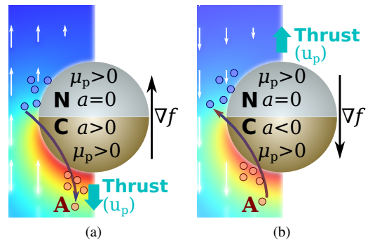
Fig. 1. Representation of Janus particle with catalytic (C) and non-catalytic (N) parts: a scheme of the catalytic reaction with, here, an homogeneous phoretic mobility \mu_p , and a surface activity in the C region that (a) a > 0 is producing A and (b) a < 0 is consuming A, that induces a gradient field, \nabla f , leading to a net swimming velocity, u_p .
