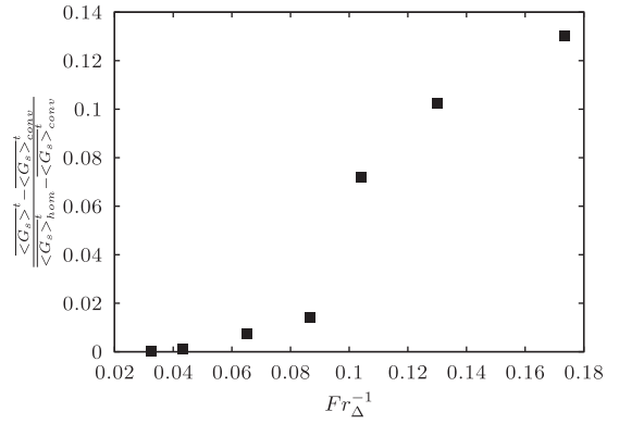
Fig. 4. Influence of mesh size on the total volumetric mass flux \langle G_s \rangle^t . In the vertical axis, hom corresponds to the homogeneous case and conv corresponds to the converged case, Fr_{\Delta}^{-1} = 0.032 .
