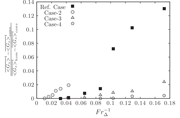
Fig. 12. Influence of mesh size on the total vertical solid mass flux \overline{\langle G_s \rangle}^t for different type of Geldart particles (for details, see Table 1). In the vertical axis, hom corresponds to the homogeneous case and conv corresponds to the converged case.
