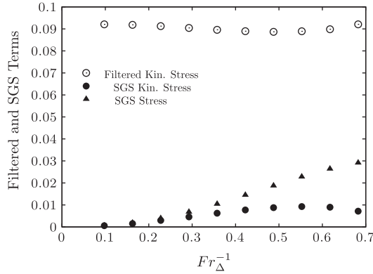
Fig. 14. Filtered and sub-grid contributions of particulate and sub-grid stress terms normalised by the gravity term for different inverse Froude numbers Fr_{\Delta}^{-1} based on the filter width \Delta .
