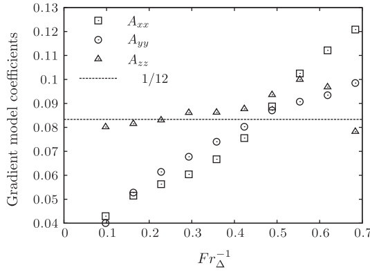
Fig. 28. Gradient model coefficients A_{\beta\beta} along the vertical ( z -) and radial ( x -, y -) directions for different inverse Froude numbers Fr_A^{-1} based on the filter width \Delta .
