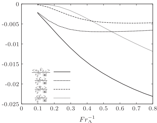
Fig. 26. Averaged Germano's decomposition terms along the mean flow direction for different inverse Froude numbers Fr_A^{-1} based on the filter width \bar{\Delta} .
