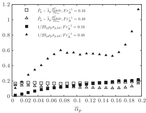
Fig. 16. Filtered particulate stress tensor trace \tilde{P}_p - \tilde{\lambda}_p \frac{\partial \tilde{U}_{p,m}}{\partial x_m} and sub-grid correlated energy 1/2\tilde{\alpha}_p \rho_p \sigma_{p,kk} conditionally averaged by filtered volume fraction for inverse Froude numbers Fr_{\Delta}^{-1} = 0.16 and Fr_{\Delta}^{-1} = 0.48 based on the filter width \bar{\Delta} (normalised \langle \tilde{\alpha}_p \rangle \rho_p (\tau_p^{st} |\mathbf{g}|)^2 ).
