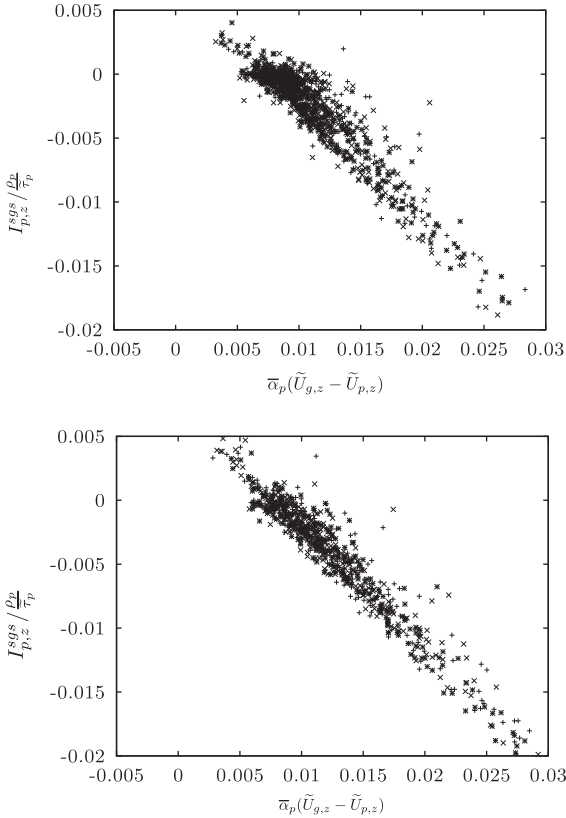
Fig. 21. Scattering plot of I_{p,z}^{sgs}/\tau_p with respect to \bar{\alpha}_p (\bar{U}_{g,z} - \bar{U}_{p,z}) for intermediate and large inverse Froude numbers Fr_A^{-1} based on the filter width \bar{\Delta} : *: Fr_A^{-1} = 0.224 , x: Fr_A^{-1} = 0.288 , +: Fr_A^{-1} = 0.416 (top) and *: Fr_A^{-1} = 0.544 , x: Fr_A^{-1} = 0.618 , +: Fr_A^{-1} = 0.683 (bottom).
