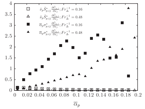
Fig. 17. Filtered particulate stress dissipation \tilde{v}_p \tilde{S}_{p,ij}^* \frac{\partial \tilde{U}_{p,i}}{\partial x_j} and sub-grid dissipation \tilde{\alpha}_p \sigma_{p,ij}^* \frac{\partial \tilde{U}_{p,i}}{\partial x_j} conditionally averaged by filtered volume fraction for inverse Froude numbers Fr_{\Delta}^{-1} = 0.16 and Fr_{\Delta}^{-1} = 0.48 based on the filter width \bar{\Delta} (normalised \langle \tilde{\alpha}_p \rangle \rho_p (\tau_p^{st} |\mathbf{g}|)^2 ).
