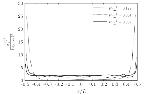
Fig. 10. Radial profile of time-averaged variance of solid volume fraction for three mesh resolutions: moderate ( 32 \times 32 \times 256 , Fr_A^{-1} = 0.128 ), fine ( 64 \times 64 \times 512 , Fr_A^{-1} = 0.064 ) and finest ( 128 \times 128 \times 1024 , Fr_A^{-1} = 0.032 ) ( z = 0.11 m, y = 0 ).
