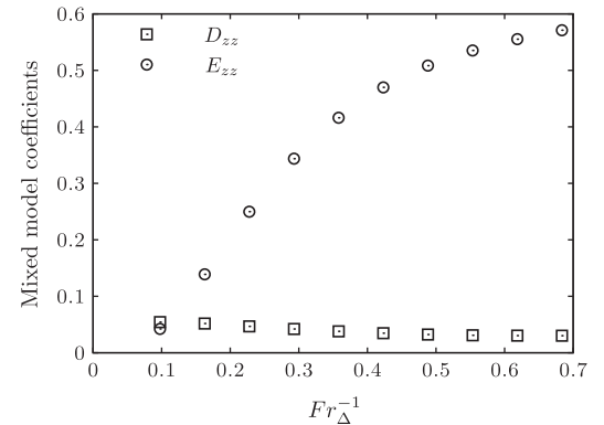
Fig. 30. Mixed model coefficients D_{zz} and E_{zz} along the mean flow for different inverse Froude numbers Fr_A^{-1} based on the filter width \Delta .
