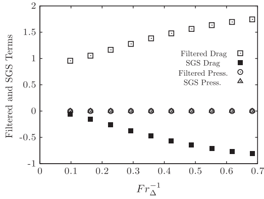
Fig. 13. Filtered and sub-grid contributions drag force and gas pressure gradient without hydrostatic part normalised by the gravity term for different inverse Froude numbers Fr_{\Delta}^{-1} based on the filter width \Delta .
