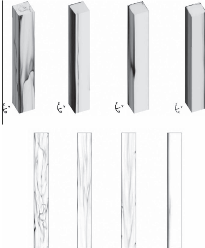
Fig. 2. Instantaneous particle volume fraction field in the periodic circulating fluidized bed for different mesh resolutions (top: 3D view, bottom: x-y plane). From left to right, the mesh resolution is decreased. White level corresponds to \alpha_p = 0 , and back level to \alpha_{p,max} = 0.64 .
