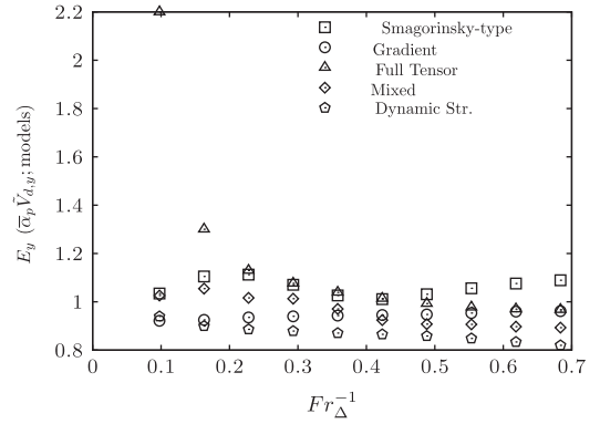
Fig. 38. Mean squared error E_y , computed as in Eq. (21), for the y-component of measured and modelled \tilde{u}_p\tilde{V}_{d,\beta} for different inverse Froude numbers Fr_A^{-1} based on the filter width \bar{\Delta} . The test filter width is \hat{\Delta} = \sqrt{5}\bar{\Delta} by following Lilly (1992).
