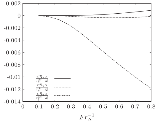
Fig. 27. Averaged Reynolds terms along the vertical (z-) and radial (x-, y-) directions for different inverse Froude numbers Fr_A^{-1} based on the filter width \bar{\Delta} .
