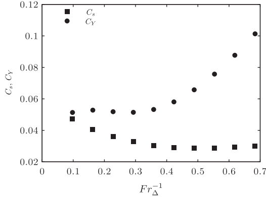
Fig. 44. Yoshizawa and Smagorinsky model coefficients, C_Y and C_s , respectively, for different inverse Froude numbers Fr_A^{-1} based on the filter width \bar{\Delta} .
