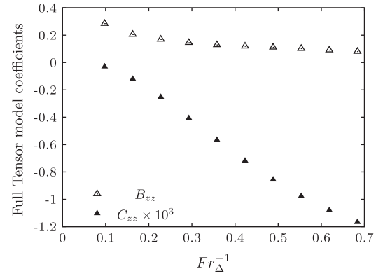
Fig. 29. Full Tensor model coefficients B_{zz} and C_{zz} along the mean flow for different inverse Froude numbers Fr_A^{-1} based on the filter width \Delta .
