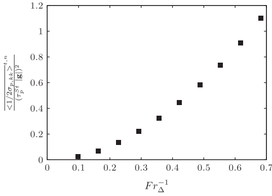
Fig. 15. Averaged sub-grid correlated energy 1/2\sigma_{p,kk} for different inverse Froude numbers Fr_{\Delta}^{-1} based on the filter width \bar{\Delta} .
