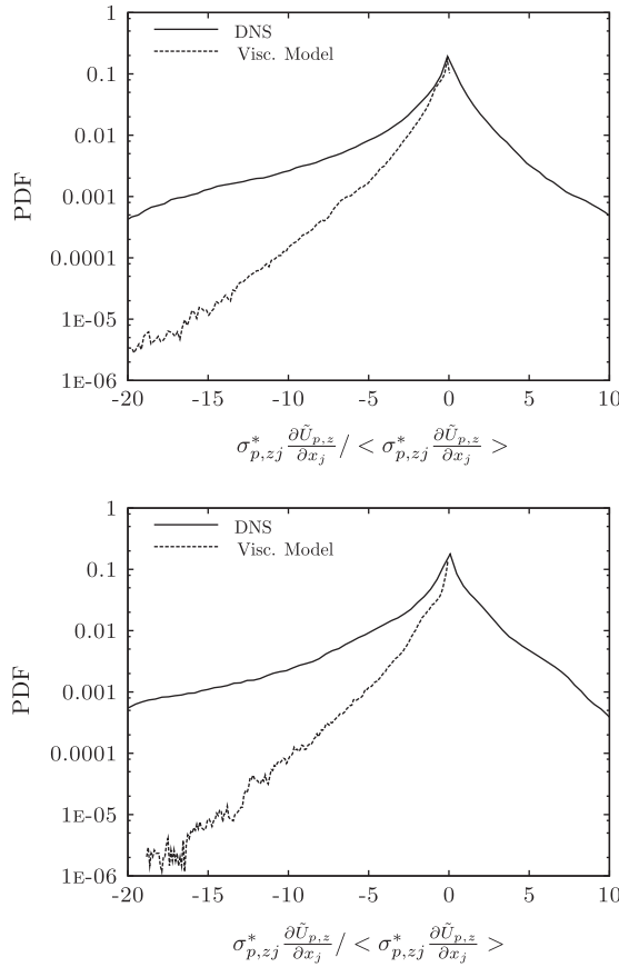
Fig. 43. Pdfs of particle sub-grid dissipation from DNS data and by the Smagorinsky model for inverse Froude numbers Fr_A^{-1} = 0.224 and 0.480 .
