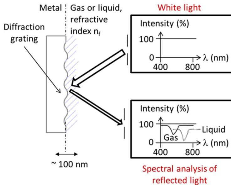
Figure 1: Reflectance of collimated TM polarized white light on a metallic grating due to Surface Plasmon Resonance
