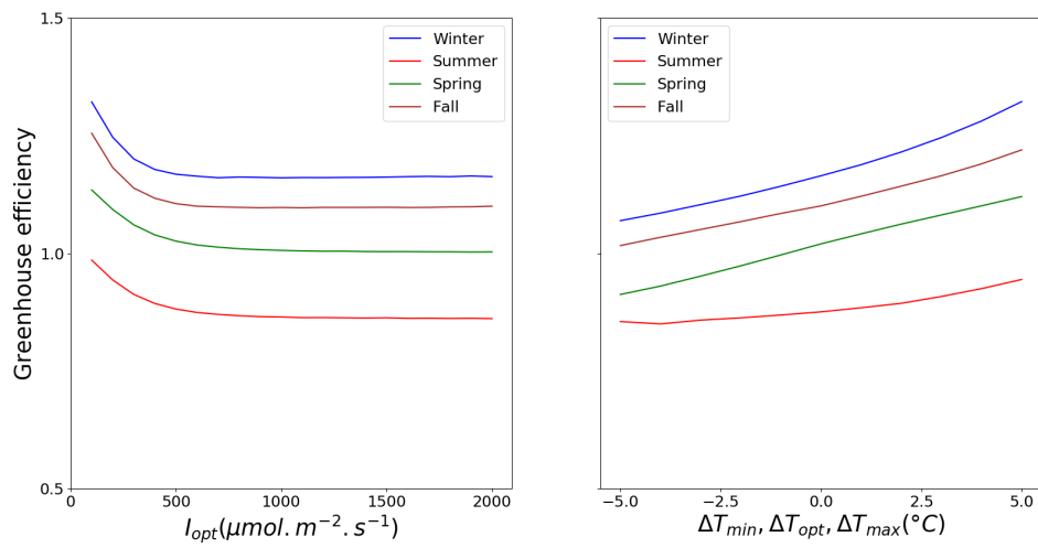
Figure 5: Greenhouse efficiency as a function of the parameter I_{opt} (left) and as a function of a shift \Delta T in all the cardinal temperatures parameters (right), for Tetraselmis suecica along different seasons of the year at a location near Nice.
