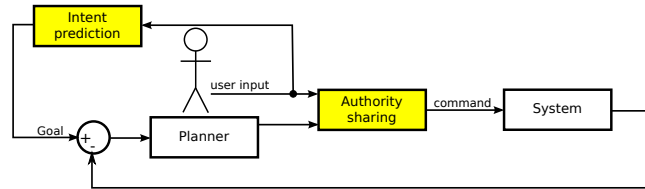
Figure 1: Sharing control model in semi-automated systems (yellow boxes are responsible for the control sharing)
