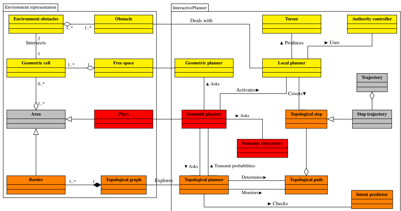
Figure 3: UML domain model of environment representation and interactive planner (red classes handle semantics, orange classes handle topology, and yellow classes handle geometry)
