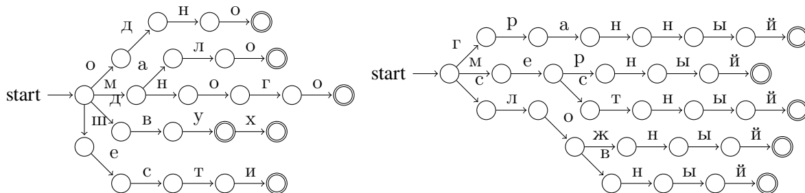
Figure 2: Left: the FSM for numerals with interfix (один ‘odin’ (one) → одно ‘odno’, два ‘dva’ (two) → дву/двух ‘dva/dvukh’, шесть ‘shest’ (six) → шести ‘shesti’, мало ‘malo’ (few) and много ‘mnogo’ (many) remain unchanged). Right: the FSM for adjectives derived from nouns грань ‘gran’ (face (of a figure)), мера ‘mera’ (measure), место ‘mesto’ (place, seat), слог ‘slog’ (syllable), слово ‘slovo’ (word) with the suffix -ный (ый) ‘-ny(y)’. The concatenated FSM with ID rule761 ([num + ITFX] + noun + н1(ый) → adj) can recognize words многомерный ‘mnogomernyy’ (multidimensional), однословный ‘odnoslovnny’ (one-word), etc. The corresponding analyses would be represented in the form ( rule761 ([num + ITFX] + noun + н1(ый) → adj), один, слово).
