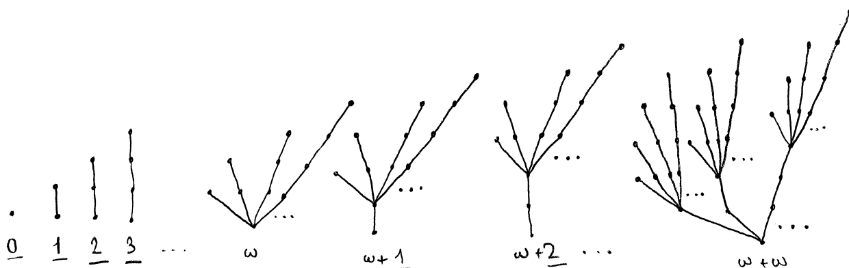
Figure 1 – Ordinal trees.
