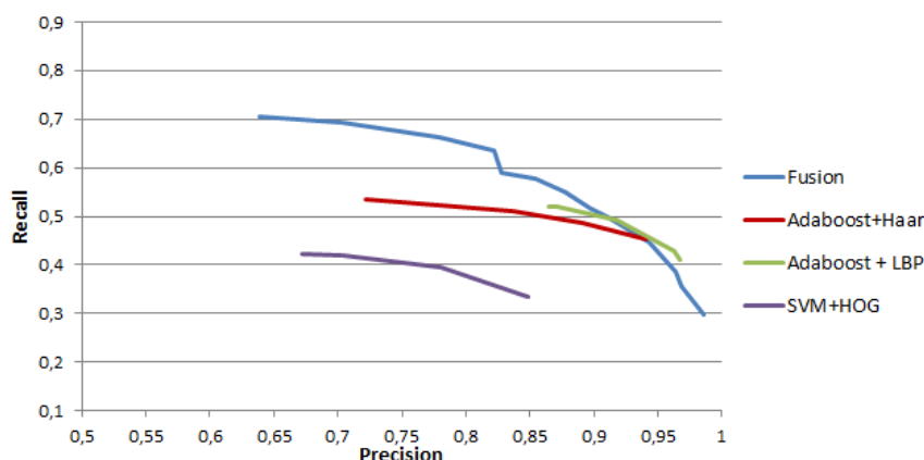
Figure 2: results of precision and recall rates
