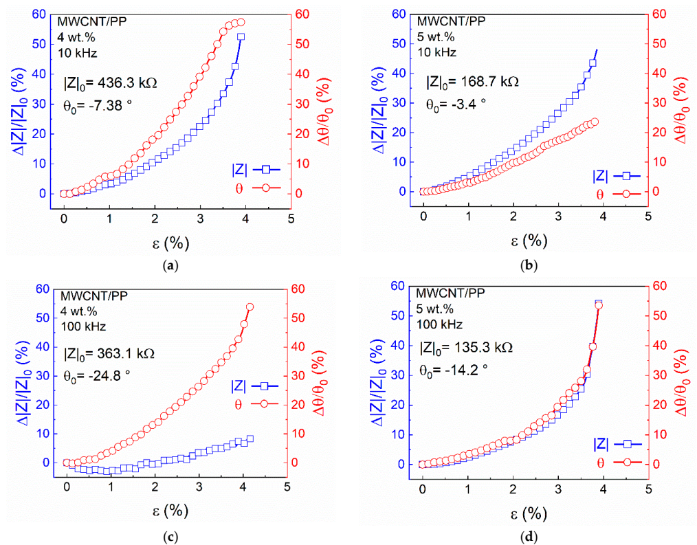
Figure 4. Piezimpedance response of nanocomposites (resistive configuration) as a function of MWCNT content and frequency. (a) 10 kHz (4 wt.%); (b) 10 kHz (5 wt.%); (c) 100 kHz (4 wt.%); (d) 100 kHz (5 wt.%).
