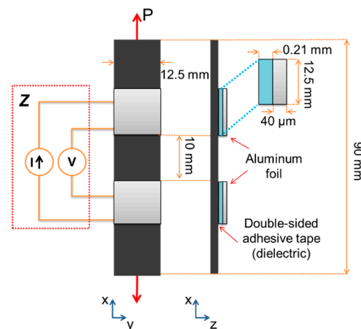
Figure 2. Specimen instrumented for piezimpedance characterization in the dielectric configuration.
