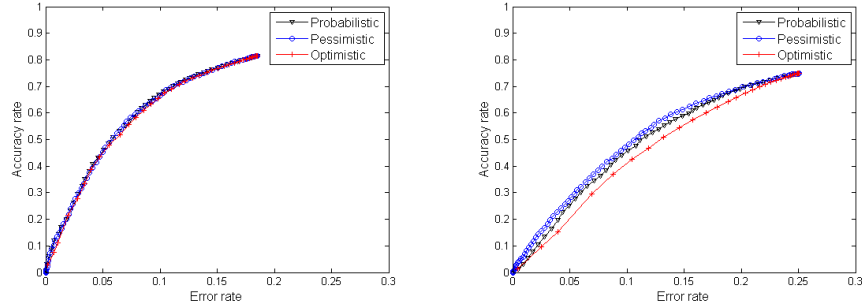
(a) Simulated data – 45 training examples (b) Simulated data – 15 training examples
